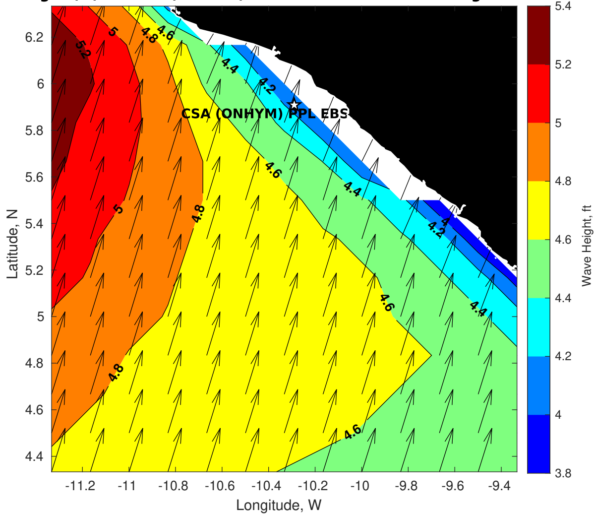
Wave Height (ft) for CSA (ONHYM) PPL EBS - Liberia at 14-Aug-2025 09:00:00
