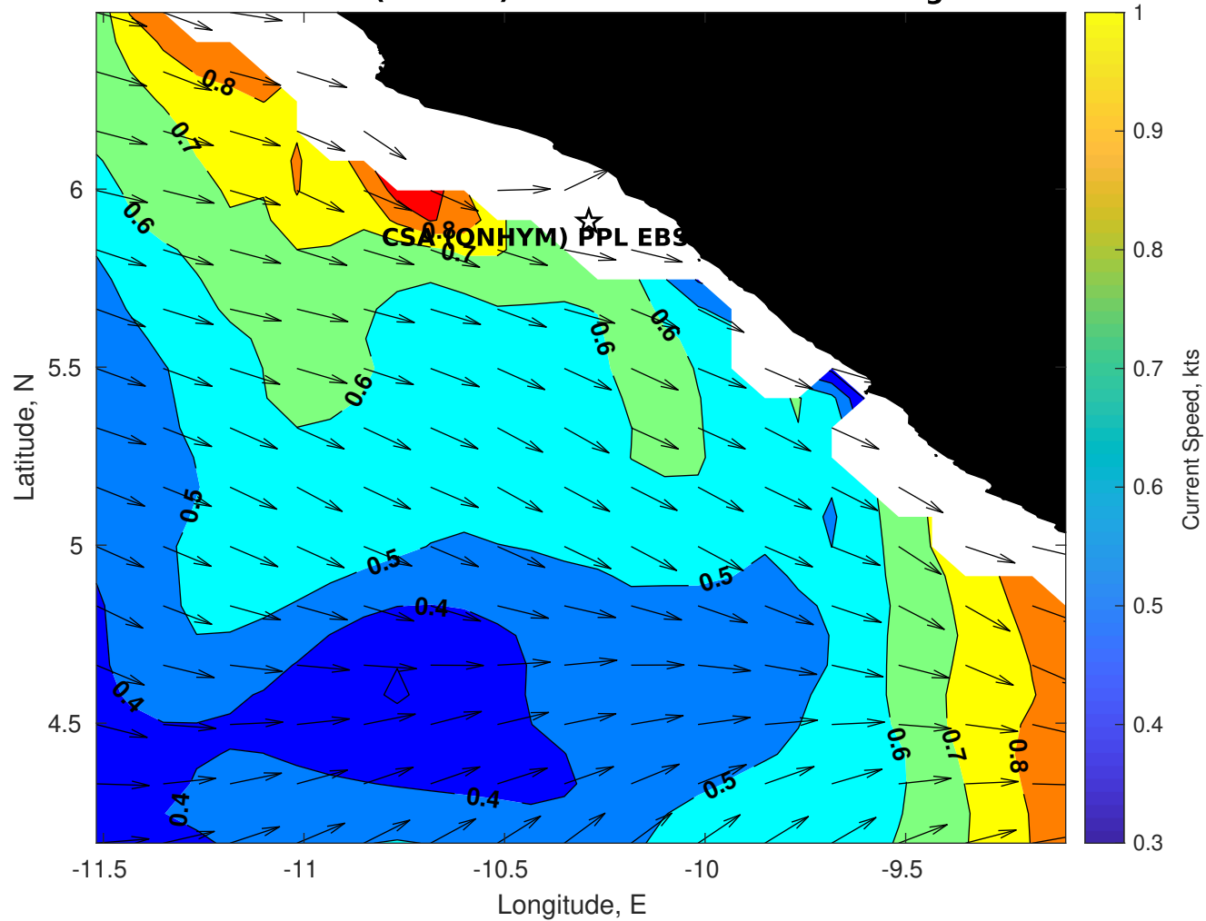
Surface Currents for CSA (ONHYM) PPL EBS - Liberia at 13-Aug-2025 00:00:00
