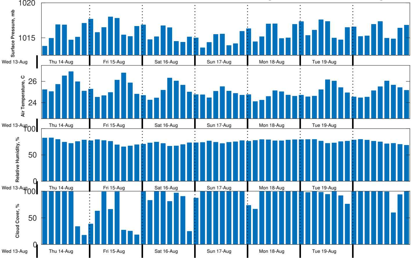
Met Forecast for CSA (ONHYM) PPL EBS - Liberia from 14-Aug-2025 00:00:00 to 21-Aug-2025 00:00:00
