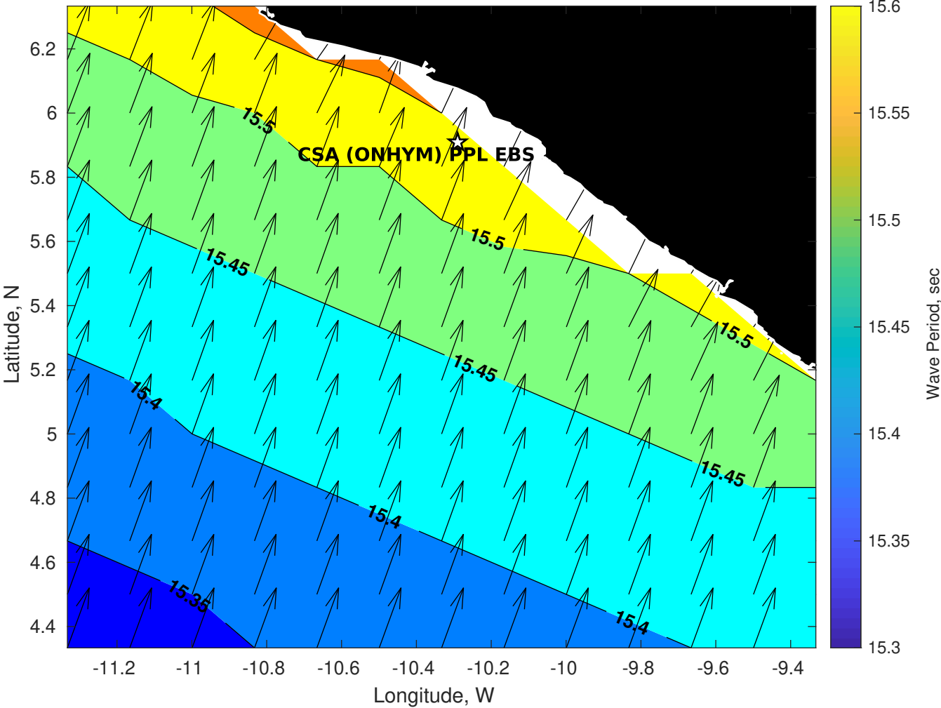
Wave Period (sec) for CSA (ONHYM) PPL EBS - Liberia at 14-Aug-2025 09:00:00
