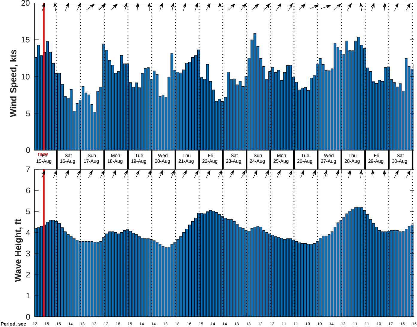
Wind & Wave Forecast for CSA (ONHYM) PPL EBS - Liberia from 14-Aug-2025 01:00:00 to 30-Aug-2025 01:00:00
