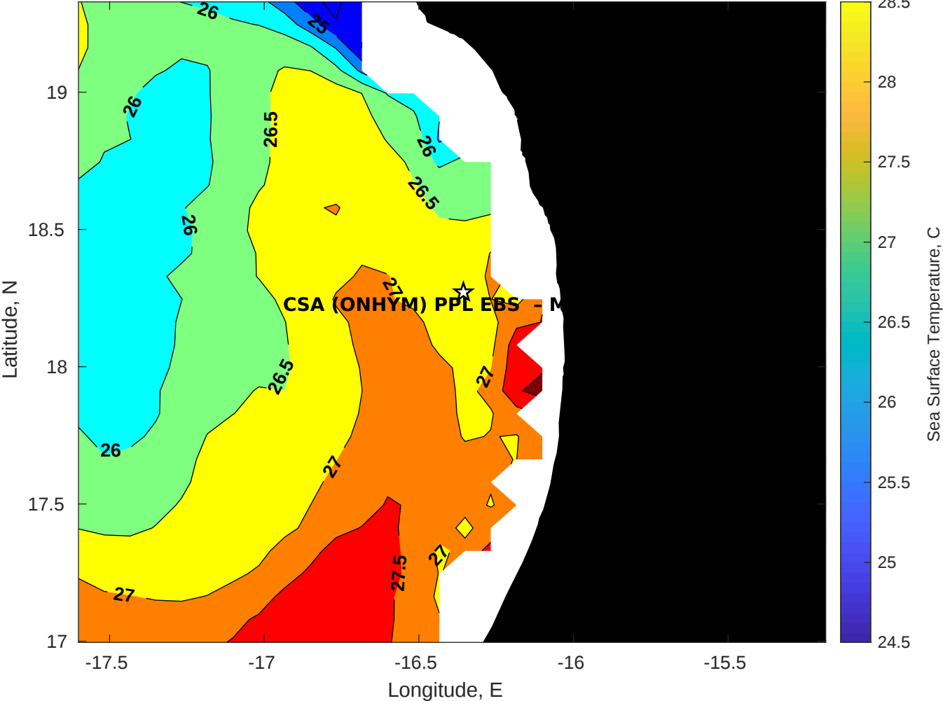
SST for CSA (ONHYM) PPL EBS - Mauritania at 13-Aug-2025 00:00:00
