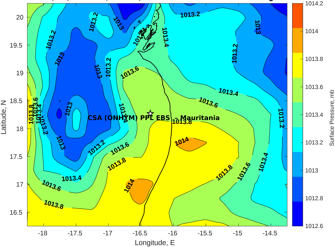
Surface Pressure (mb) for CSA (ONHYM) PPL EBS - Mauritania at 15-Aug-2025 00:00:00
