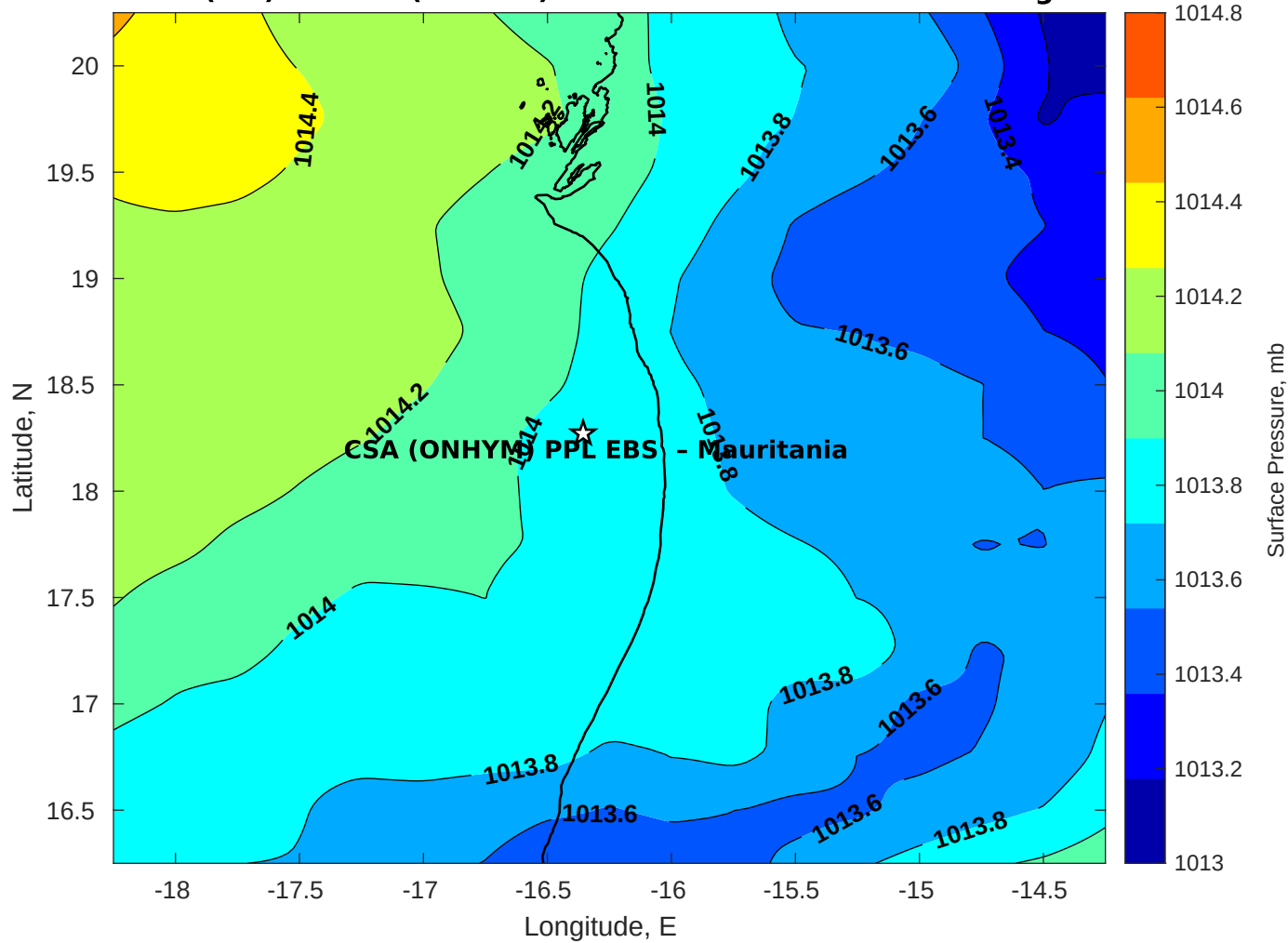
Surface Pressure (mb) for CSA (ONHYM) PPL EBS - Mauritania at 16-Aug-2025 00:00:00
