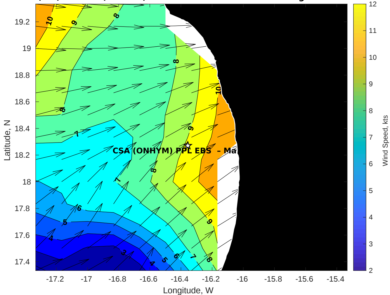
Winds (kts) for CSA (ONHYM) PPL EBS - Mauritania at 14-Aug-2025 09:00:00
