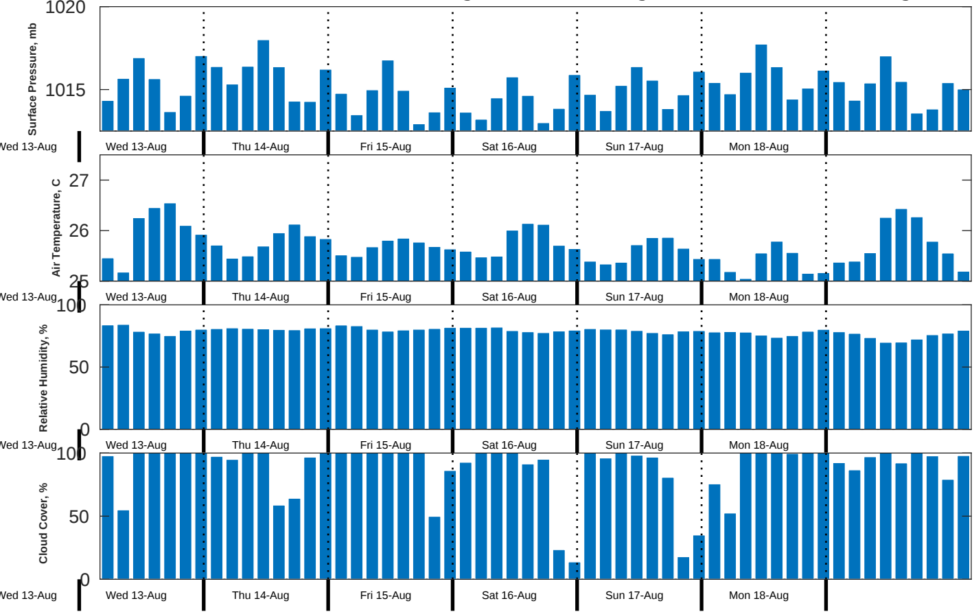
Met Forecast for CSA (ONHYM) PPL EBS - Nigeria from 14-Aug-2025 00:00:00 to 21-Aug-2025 00:00:00
