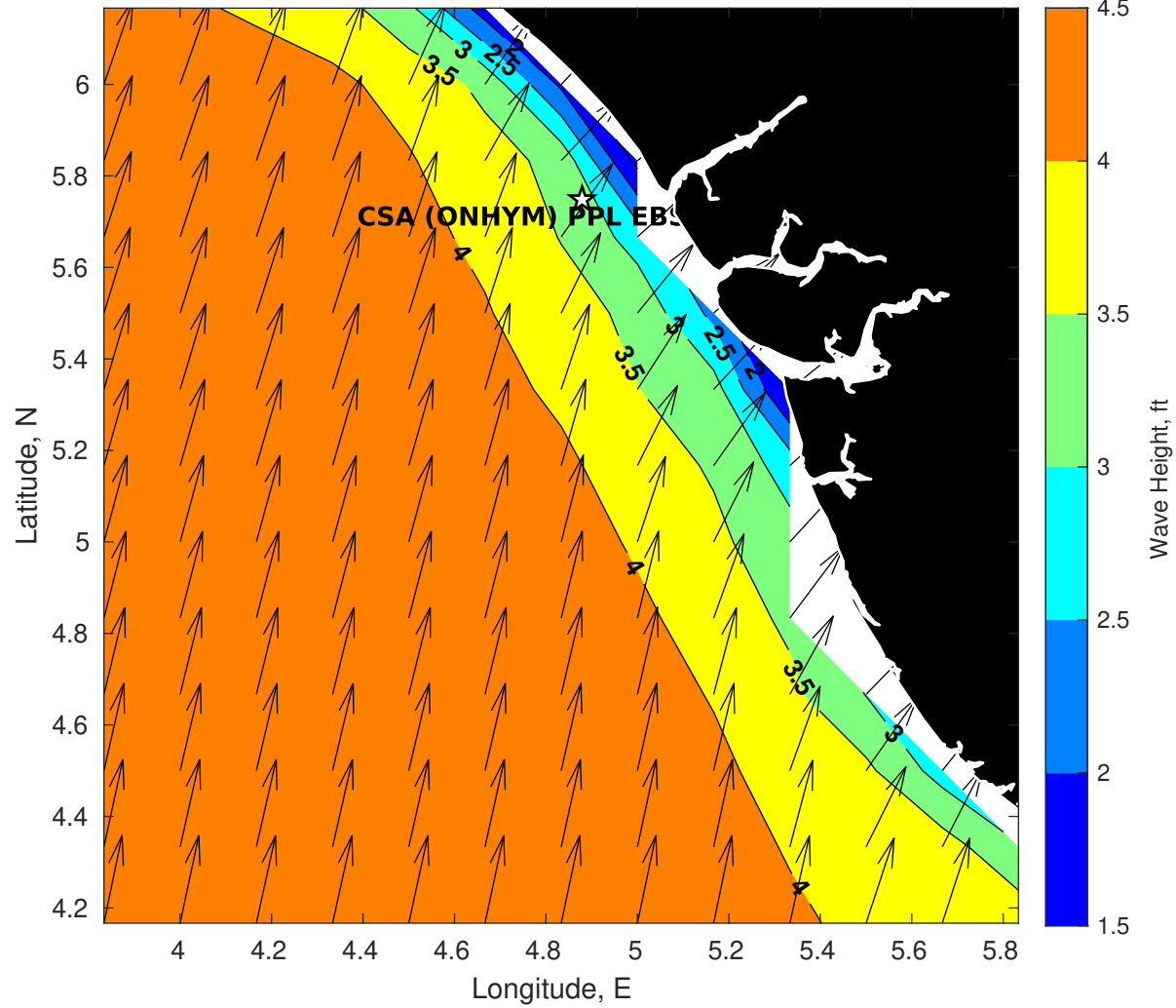
Wave Height (ft) for CSA (ONHYM) PPL EBS - Nigeria at 14-Aug-2025 09:00:00
