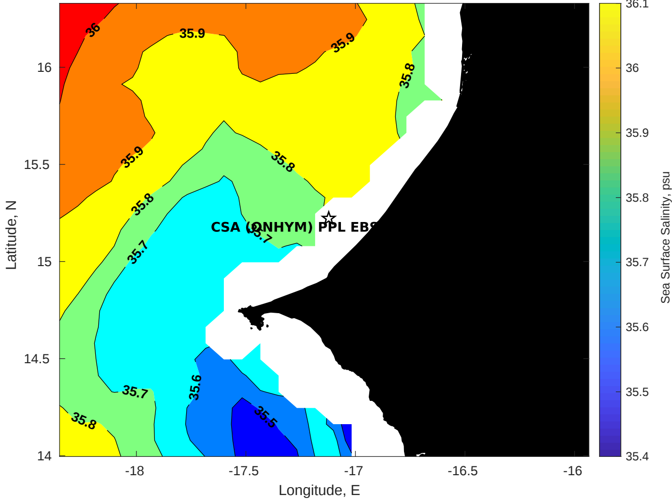
Surface Salinity for CSA (ONHYM) PPL EBS - Senegal at 13-Aug-2025 00:00:00
