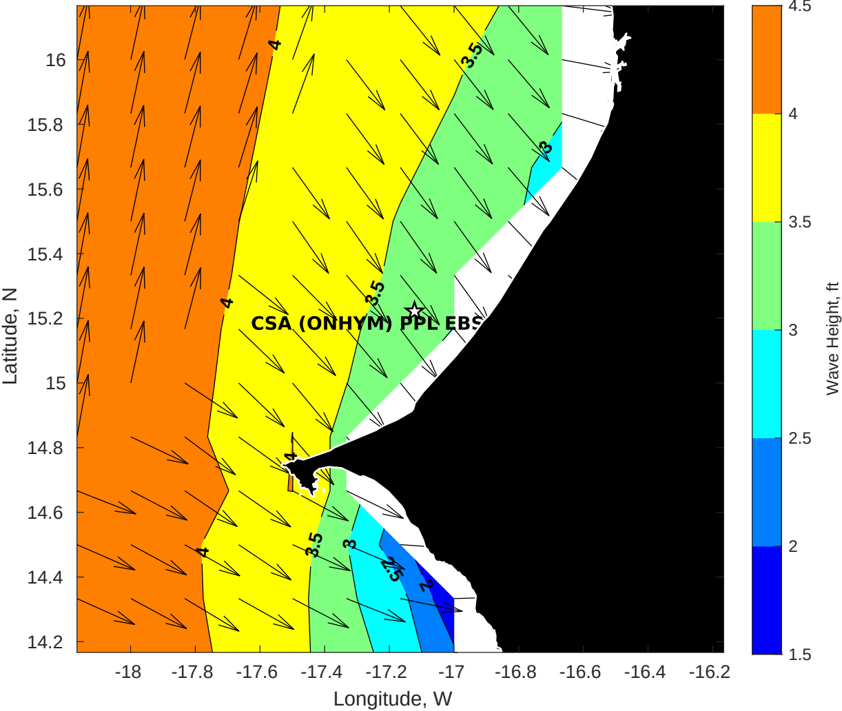
Wave Height (ft) for CSA (ONHYM) PPL EBS - Senegal at 14-Aug-2025 09:00:00
