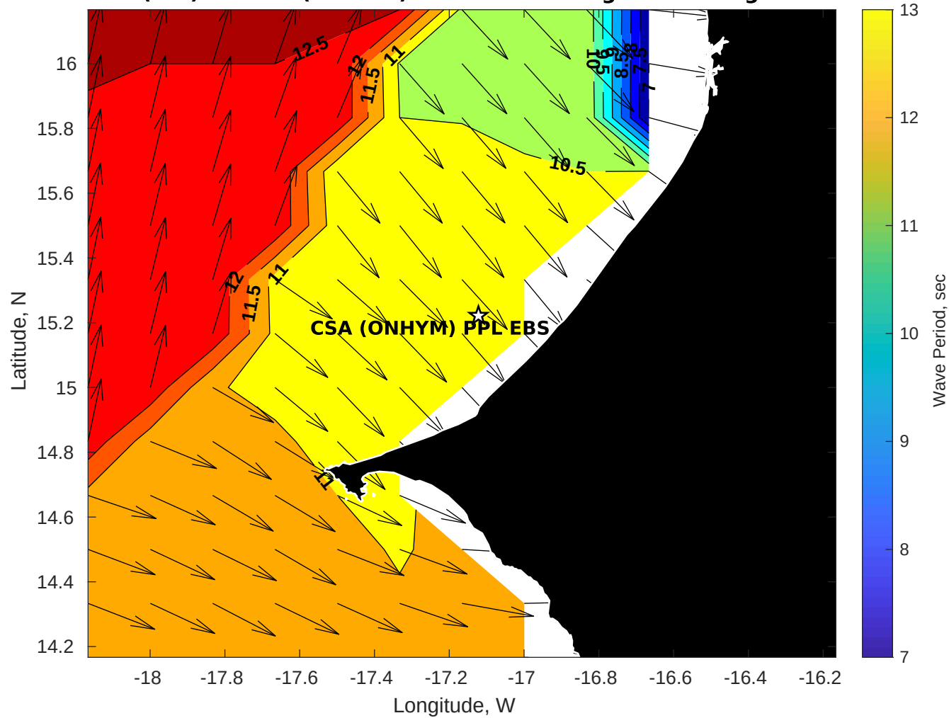
Wave Period (sec) for CSA (ONHYM) PPL EBS - Senegal at 14-Aug-2025 09:00:00
