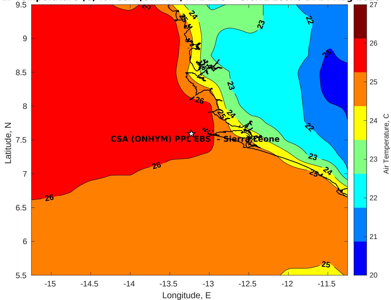
Air Temperature (C) for CSA (ONHYM) PPL EBS - Sierra Leone at 14-Aug-2025
