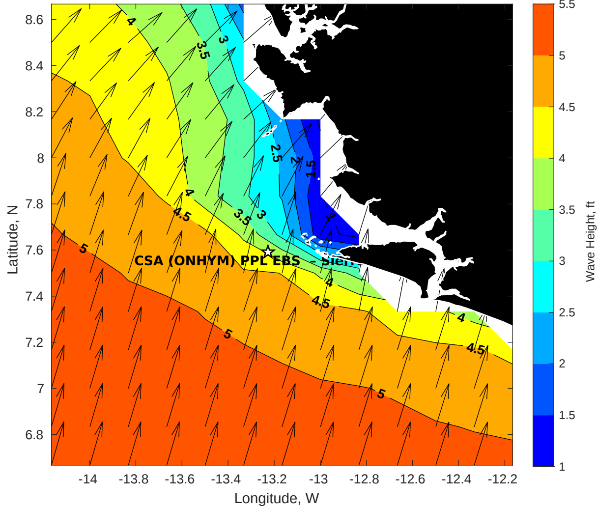
Wave Height (ft) for CSA (ONHYM) PPL EBS - Sierra Leone at 14-Aug-2025 09:00:00
