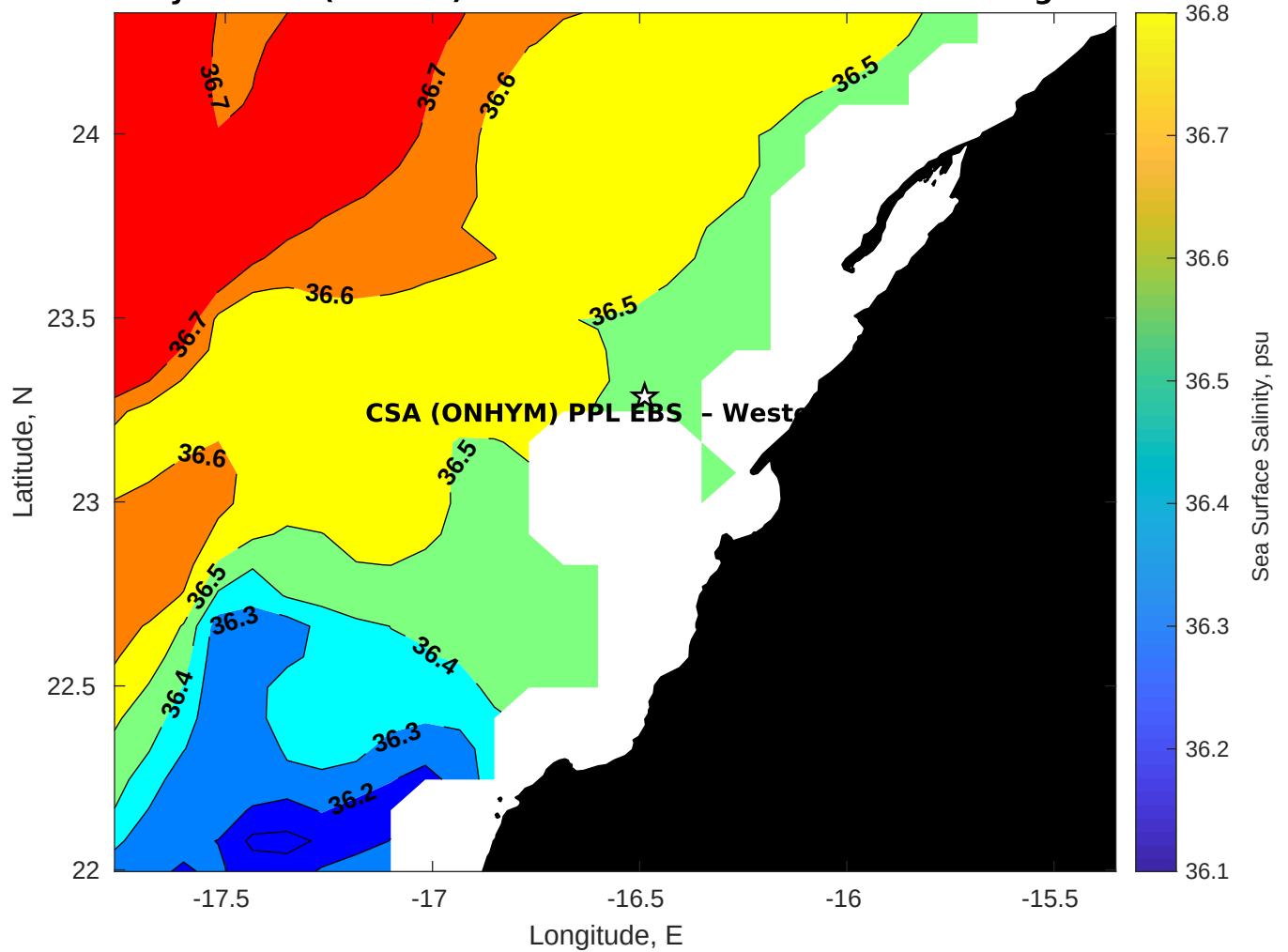
Surface Salinity for CSA (ONHYM) PPL EBS - Western Sahara at 13-Aug-2025 00:00:00
