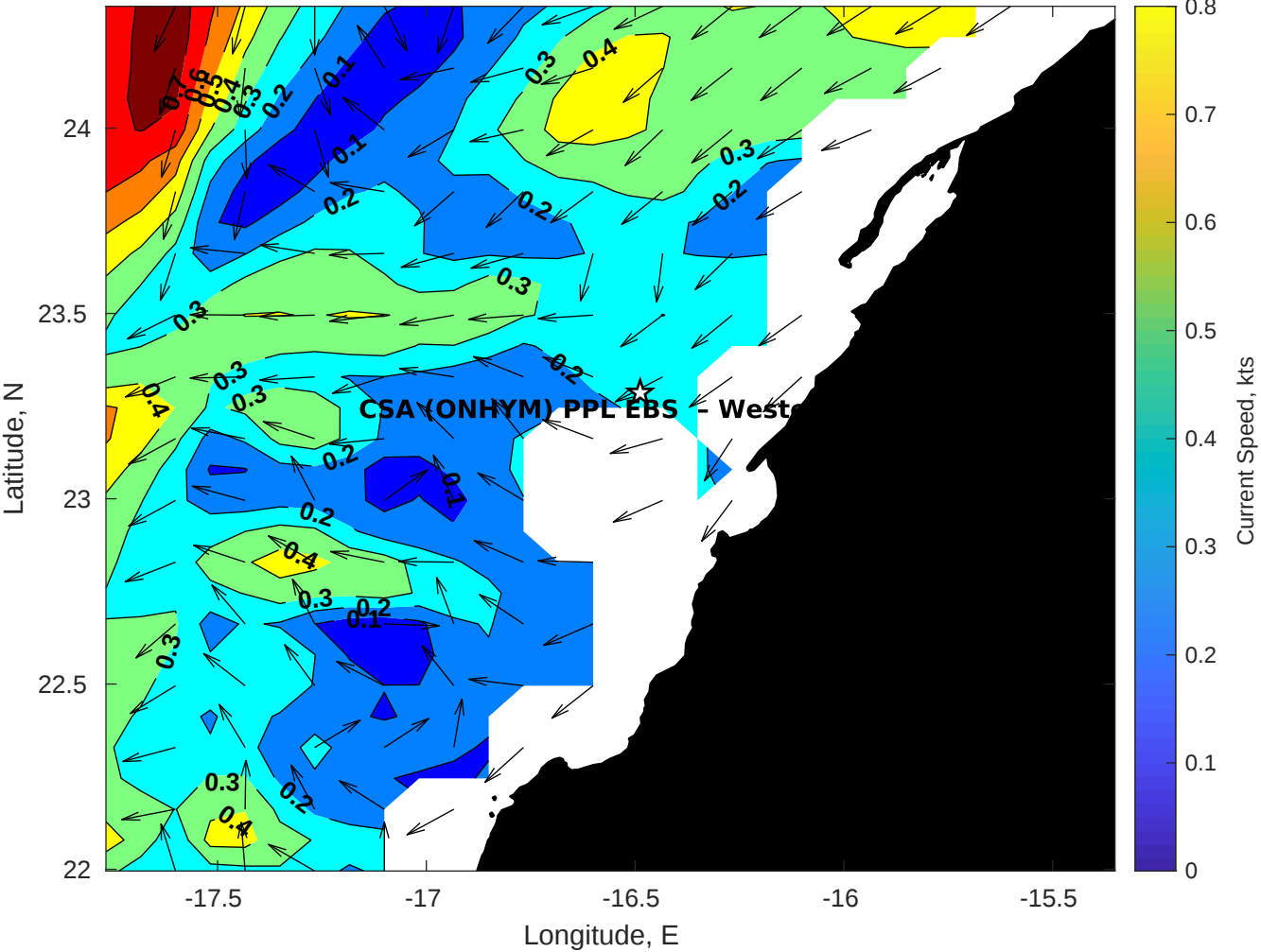
Surface Currents for CSA (ONHYM) PPL EBS - Western Sahara at 13-Aug-2025 00:00:00
