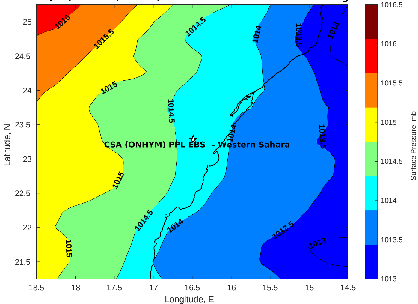
Surface Pressure (mb) for CSA (ONHYM) PPL EBS - Western Sahara at 16-Aug-2025 00:00:00
