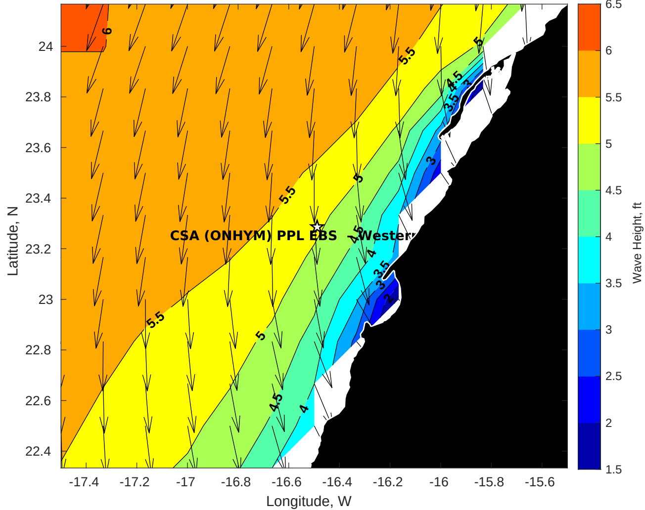
Wave Height (ft) for CSA (ONHYM) PPL EBS - Western Sahara at 14-Aug-2025 09:00:00
