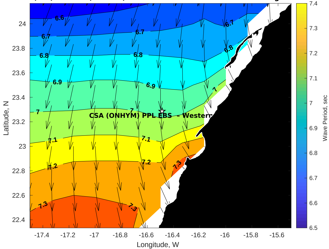
Wave Period (sec) for CSA (ONHYM) PPL EBS - Western Sahara at 14-Aug-2025 09:00:00
