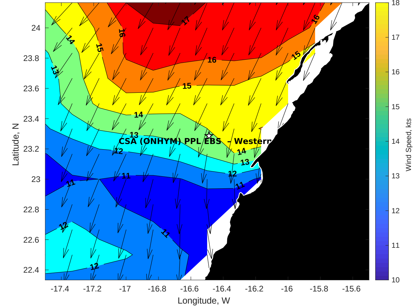
Winds (kts) for CSA (ONHYM) PPL EBS - Western Sahara at 14-Aug-2025 09:00:00
