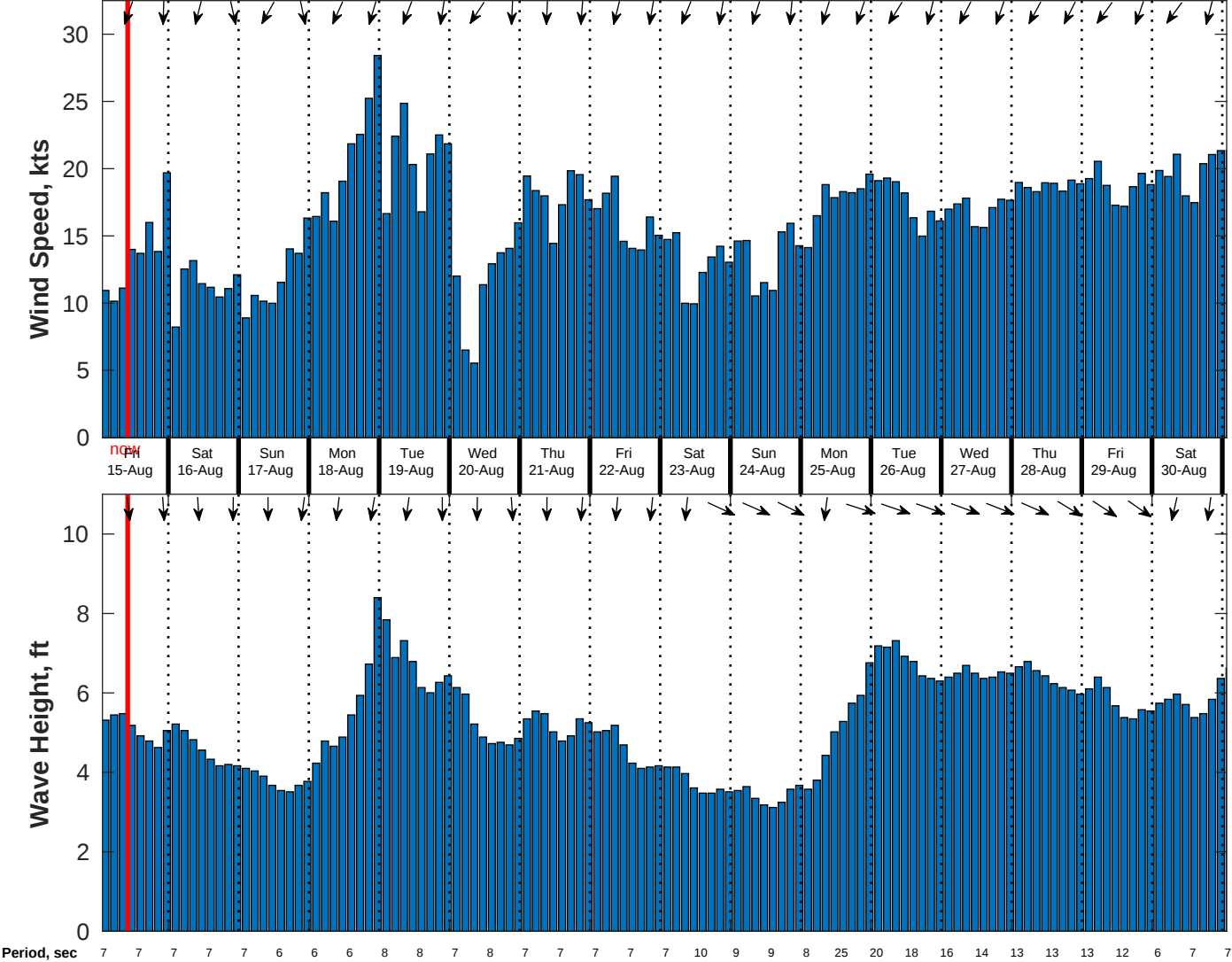
Wind & Wave Forecast for CSA (ONHYM) PPL EBS - Western Sahara from 14-Aug-2025 01:00:00 to 30-Aug-2025 01:00:00
