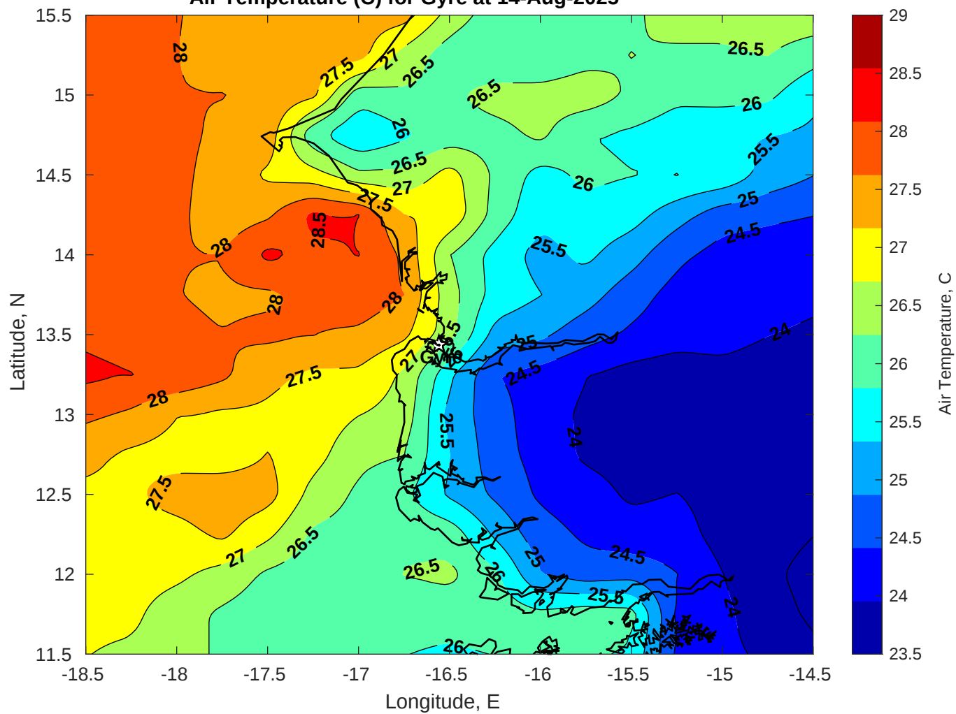
Air Temperature (C) for Gyre at 14-Aug-2025
