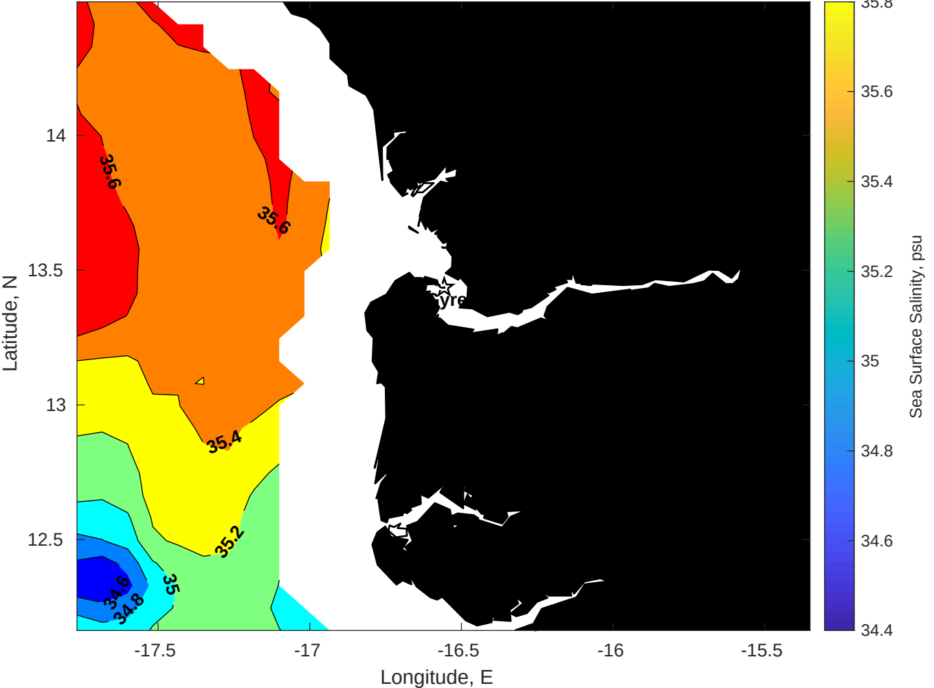
Surface Salinity for Gyre at 13-Aug-2025 00:00:00
