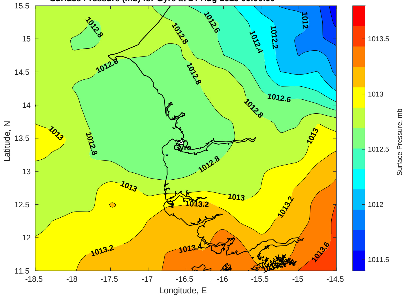
Surface Pressure (mb) for Gyre at 14-Aug-2025 00:00:00
