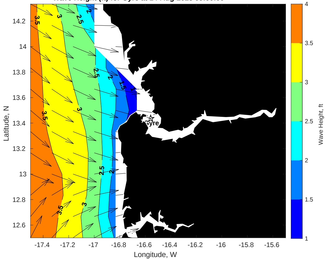
Wave Height (ft) for Gyre at 14-Aug-2025 09:00:00
