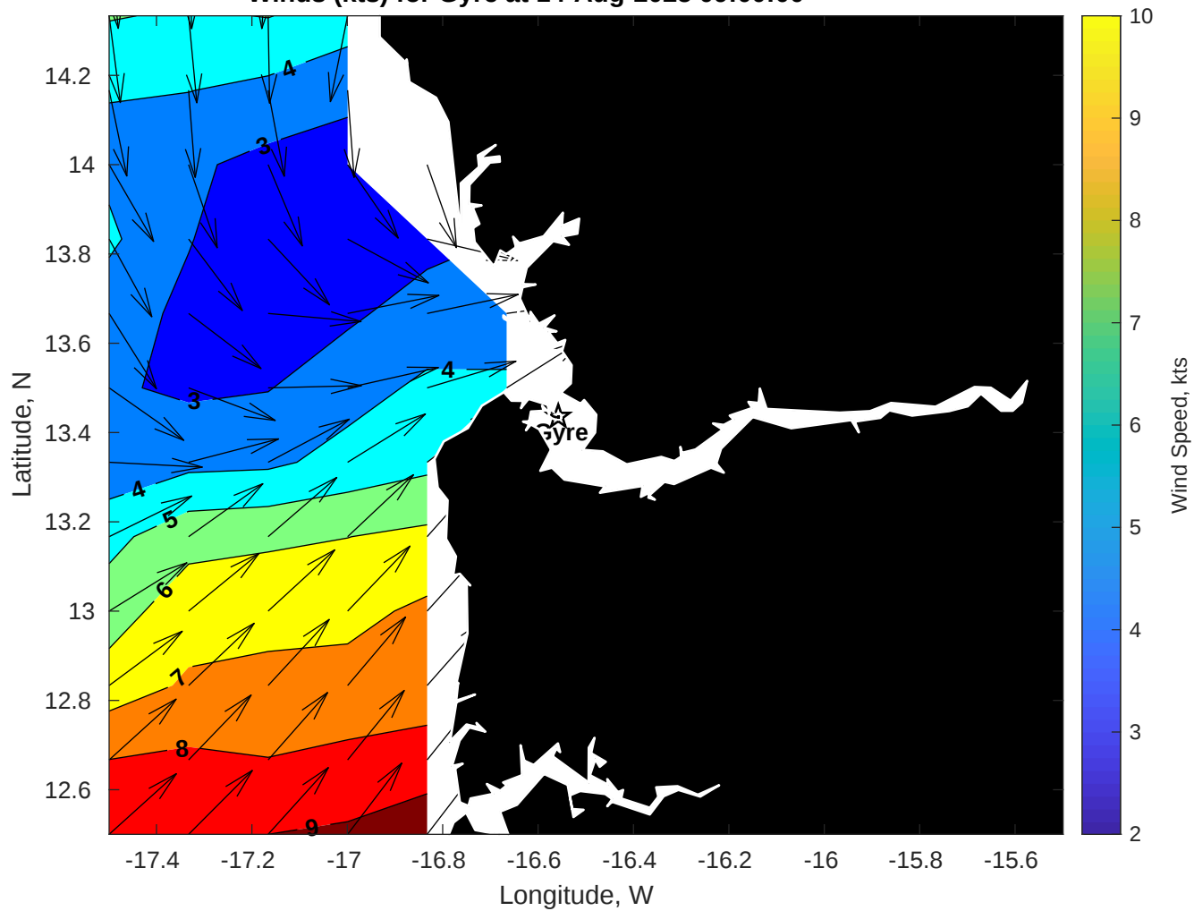
Winds (kts) for Gyre at 14-Aug-2025 09:00:00
