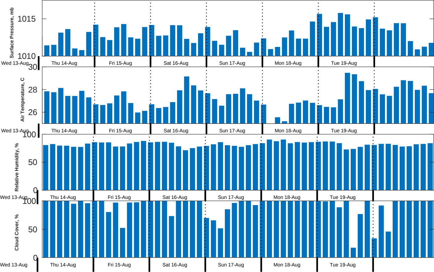
Met Forecast for Gyre from 13-Aug-2025 23:00:00 to 20-Aug-2025 23:00:00
