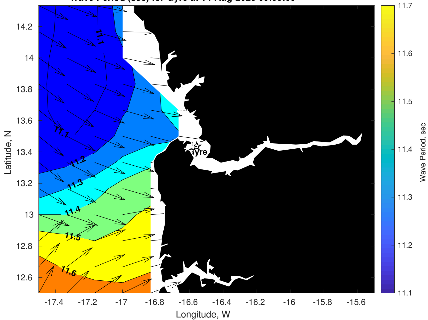
Wave Period (sec) for Gyre at 14-Aug-2025 09:00:00
