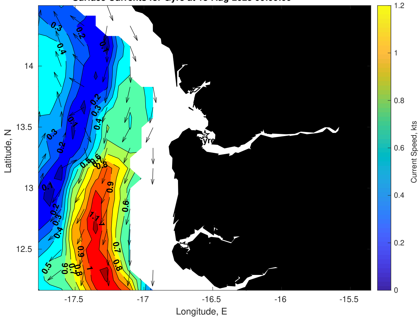
Surface Currents for Gyre at 13-Aug-2025 00:00:00
