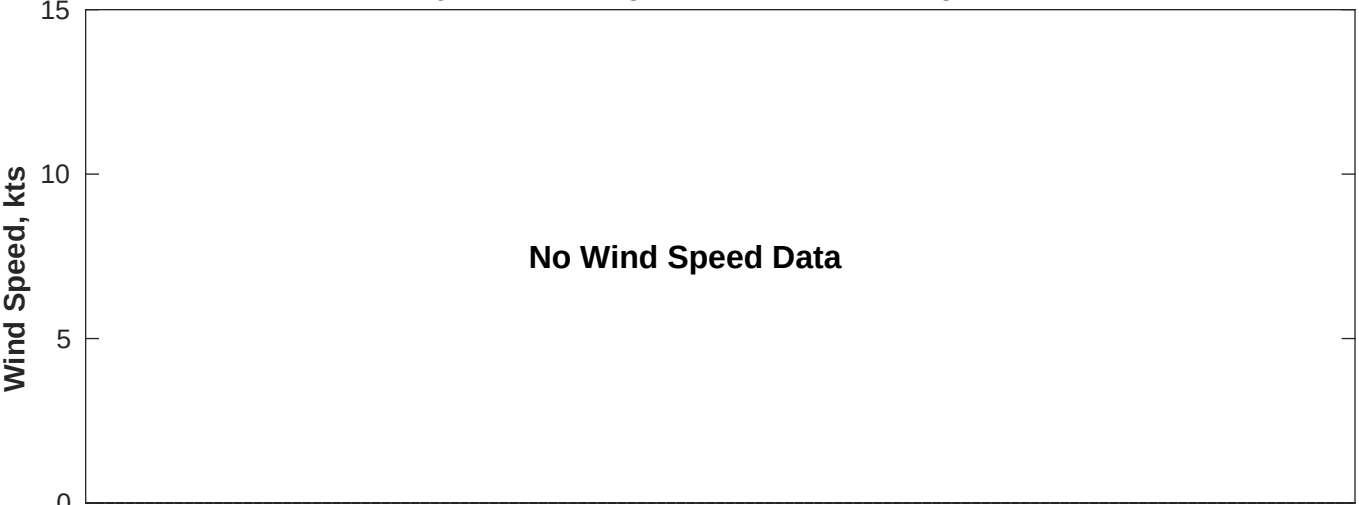
Wind & Wave Forecast for Gyre from 13-Aug-2025 23:00:00 to 29-Aug-2025 23:00:00
