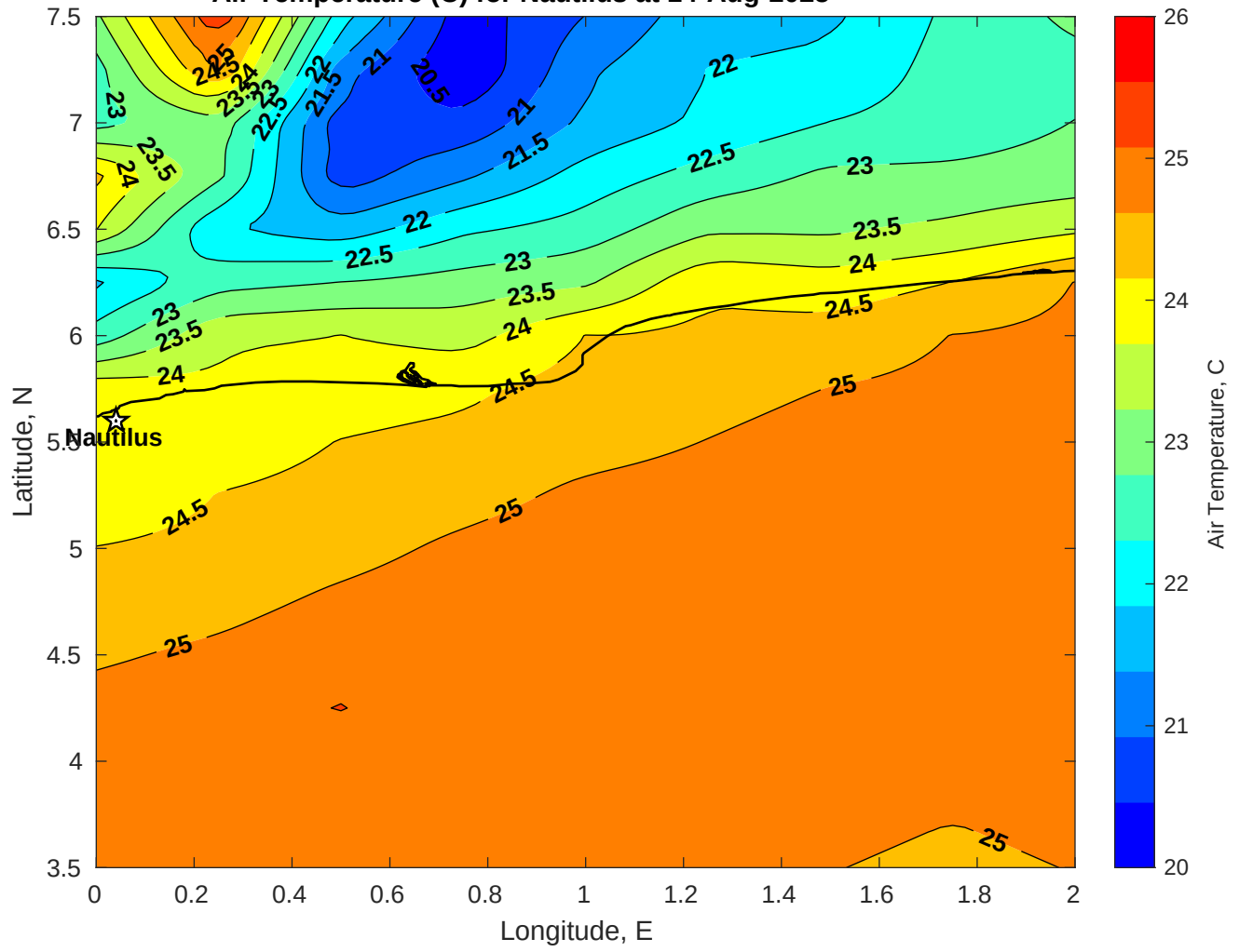
Air Temperature (C) for Nautilus at 14-Aug-2025
