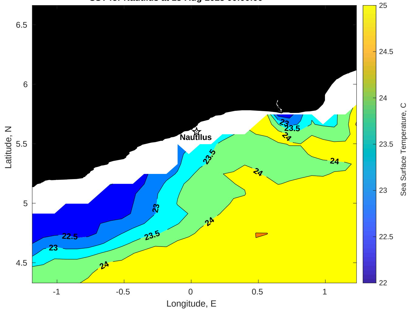
SST for Nautilus at 13-Aug-2025 00:00:00
