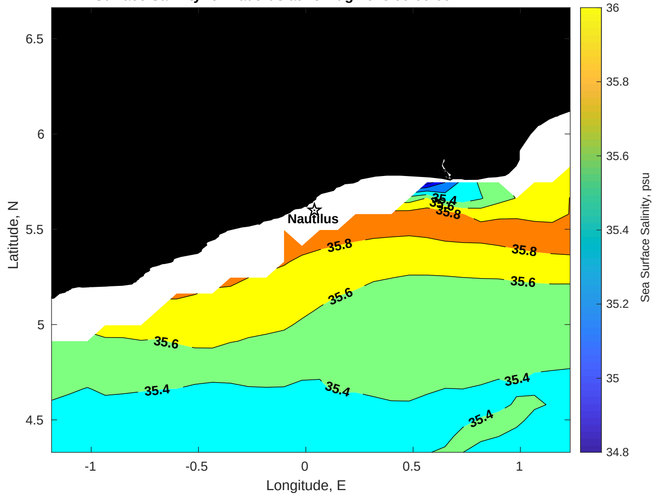
Surface Salinity for Nautilus at 13-Aug-2025 00:00:00
