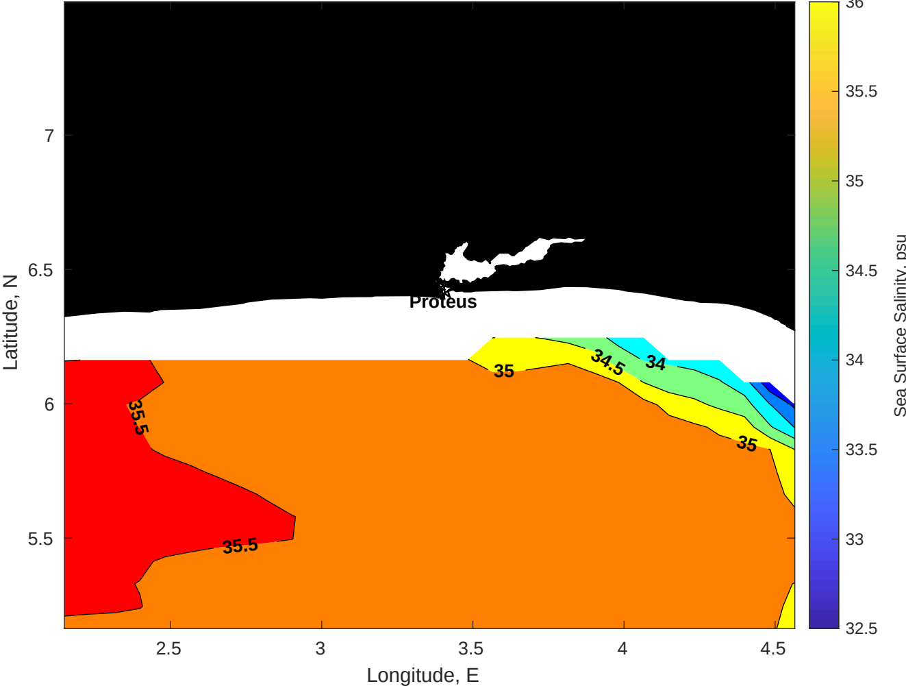
Surface Salinity for Proteus at 13-Aug-2025 00:00:00
