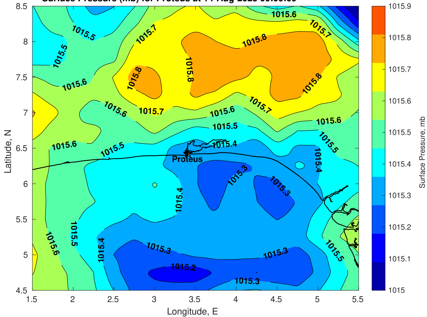
Surface Pressure (mb) for Proteus at 14-Aug-2025 00:00:00
