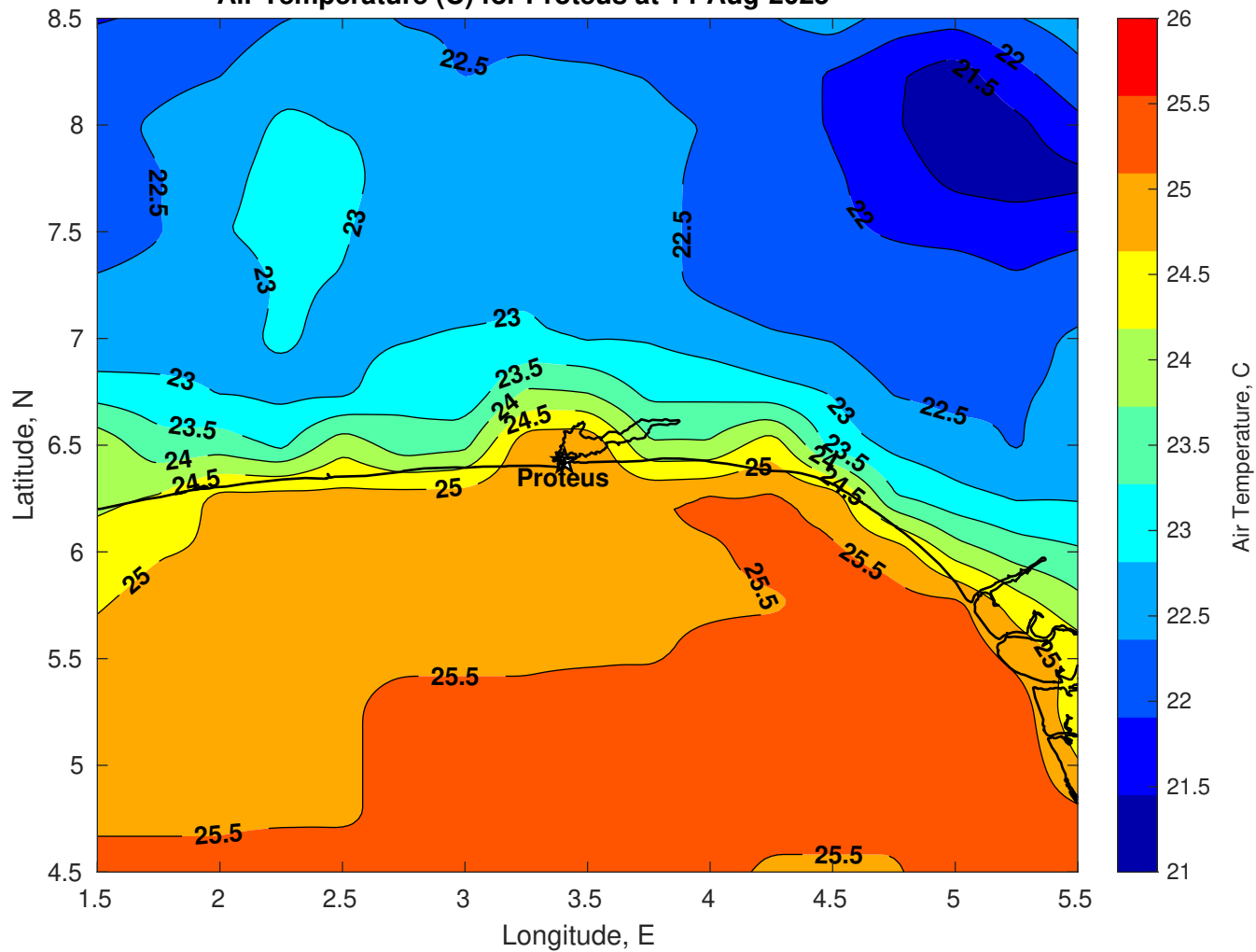
Air Temperature (C) for Proteus at 14-Aug-2025
