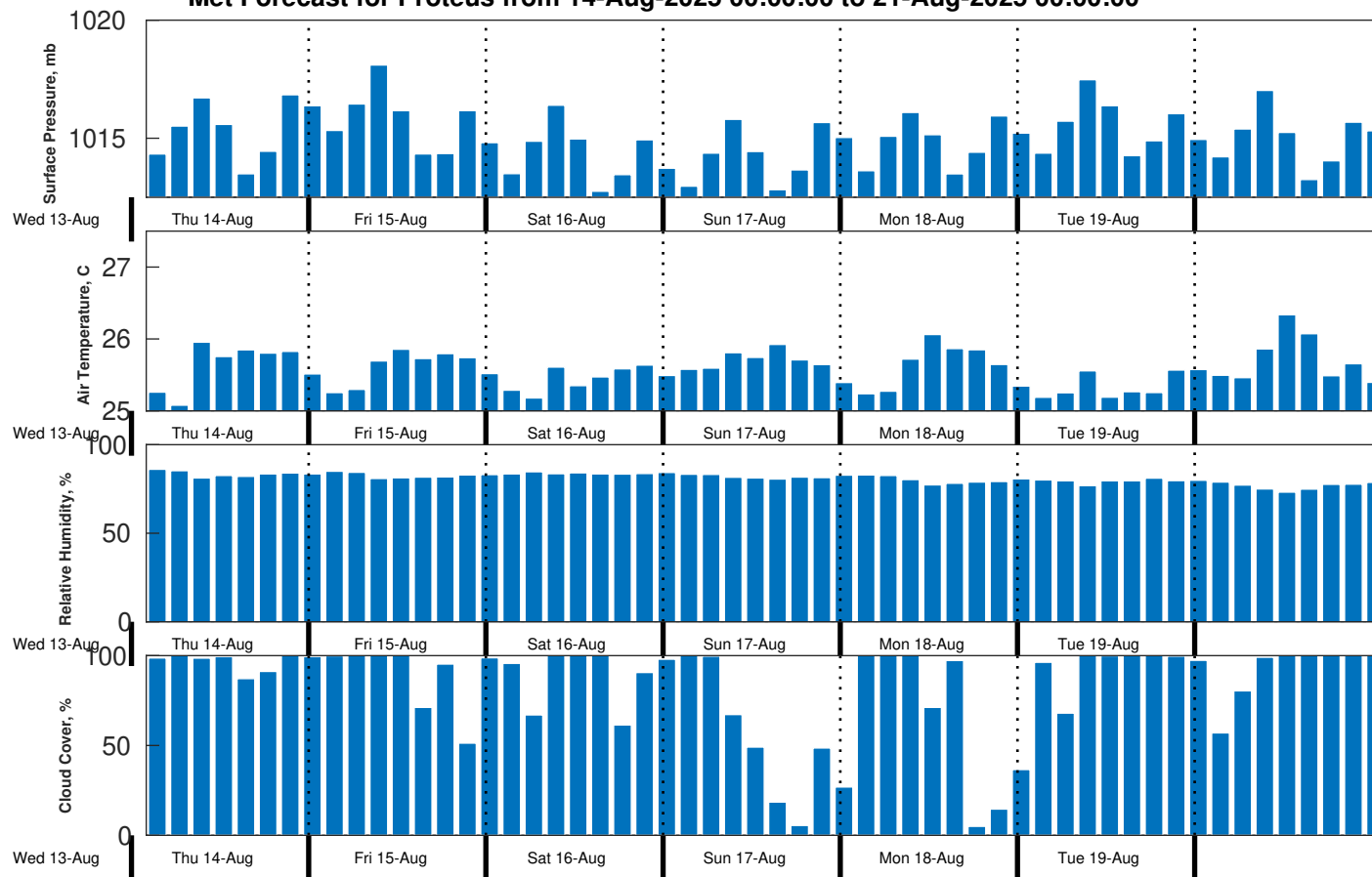
Met Forecast for Proteus from 14-Aug-2025 00:00:00 to 21-Aug-2025 00:00:00
