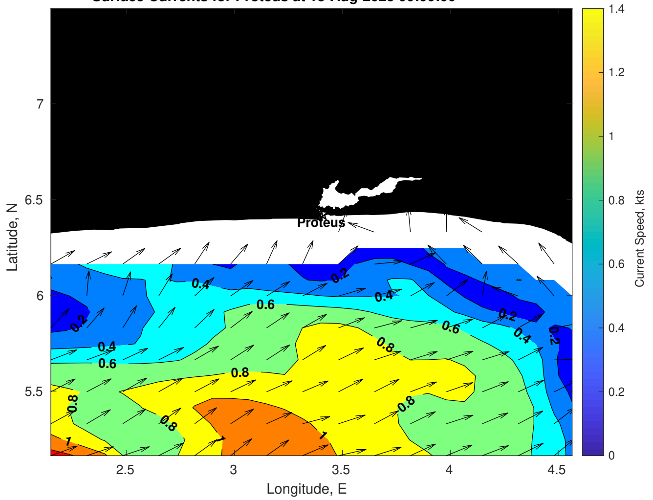
Surface Currents for Proteus at 13-Aug-2025 00:00:00
