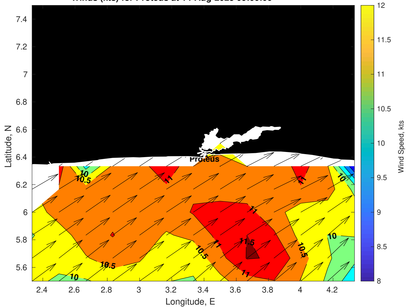
Winds (kts) for Proteus at 14-Aug-2025 09:00:00
