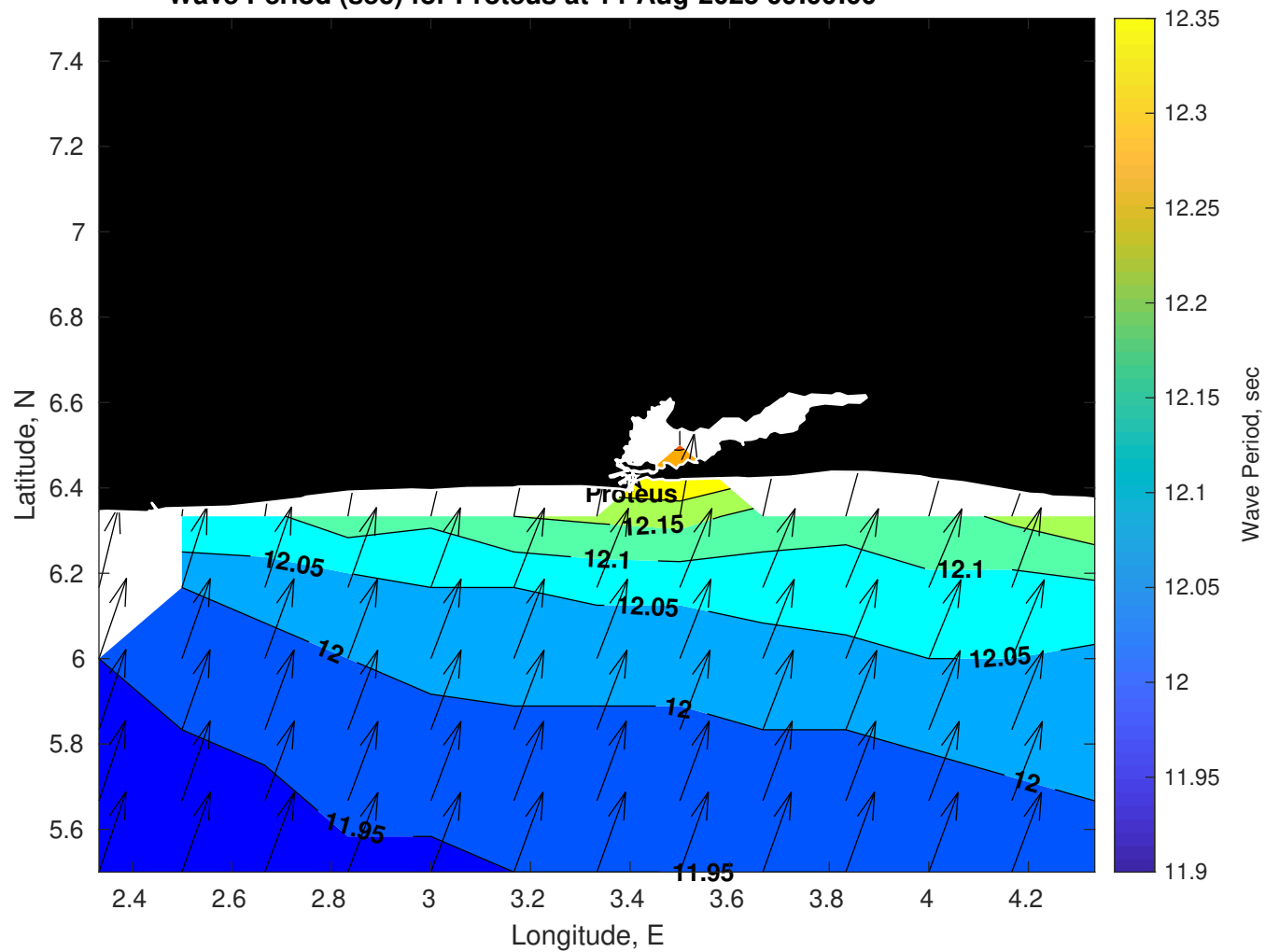
Wave Period (sec) for Proteus at 14-Aug-2025 09:00:00
