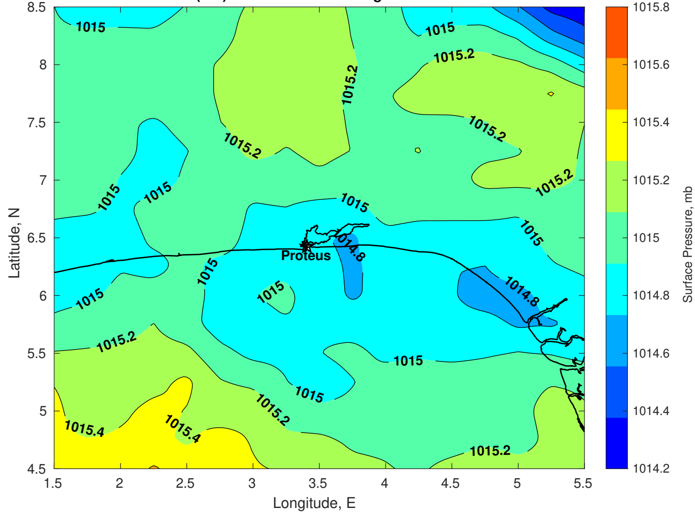
Surface Pressure (mb) for Proteus at 16-Aug-2025 00:00:00
