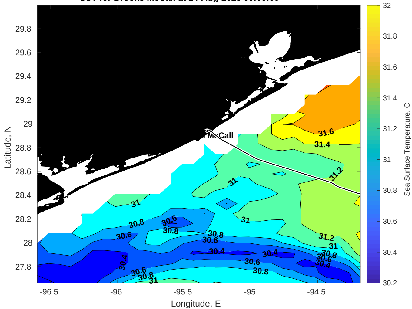
SST for Brooks McCall at 14-Aug-2025 00:00:00
