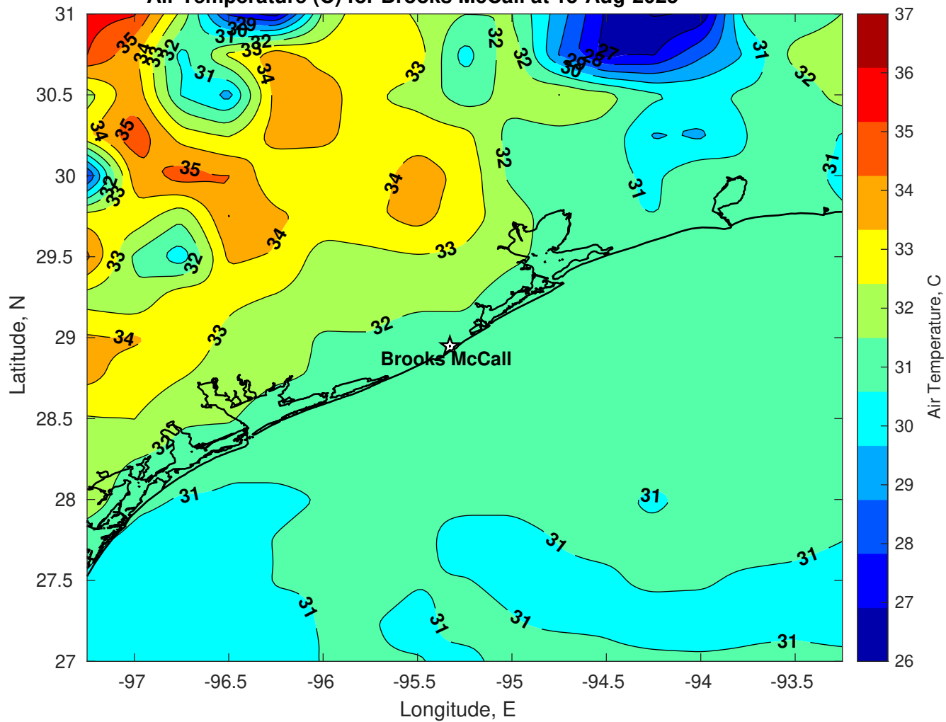
Air Temperature (C) for Brooks McCall at 15-Aug-2025
