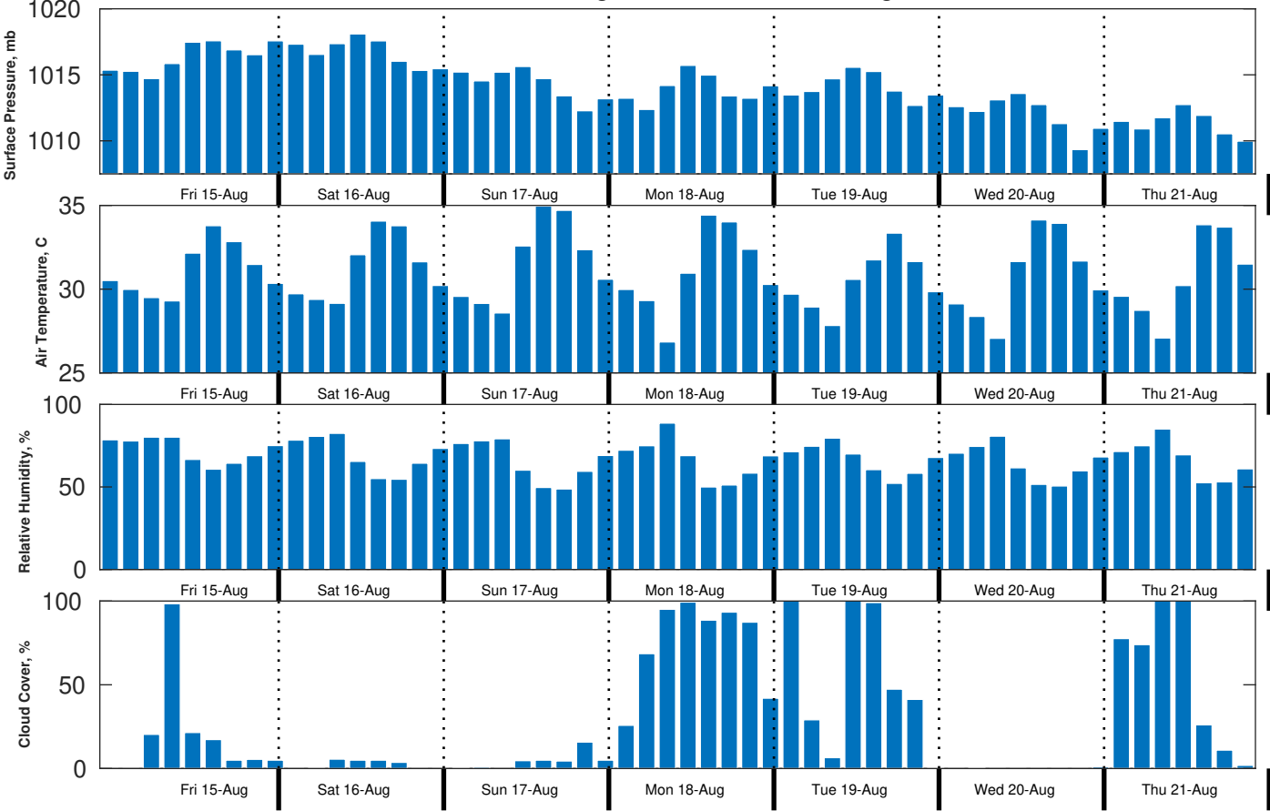
Met Forecast for Brooks McCall from 15-Aug-2025 00:00:00 to 22-Aug-2025 00:00:00
