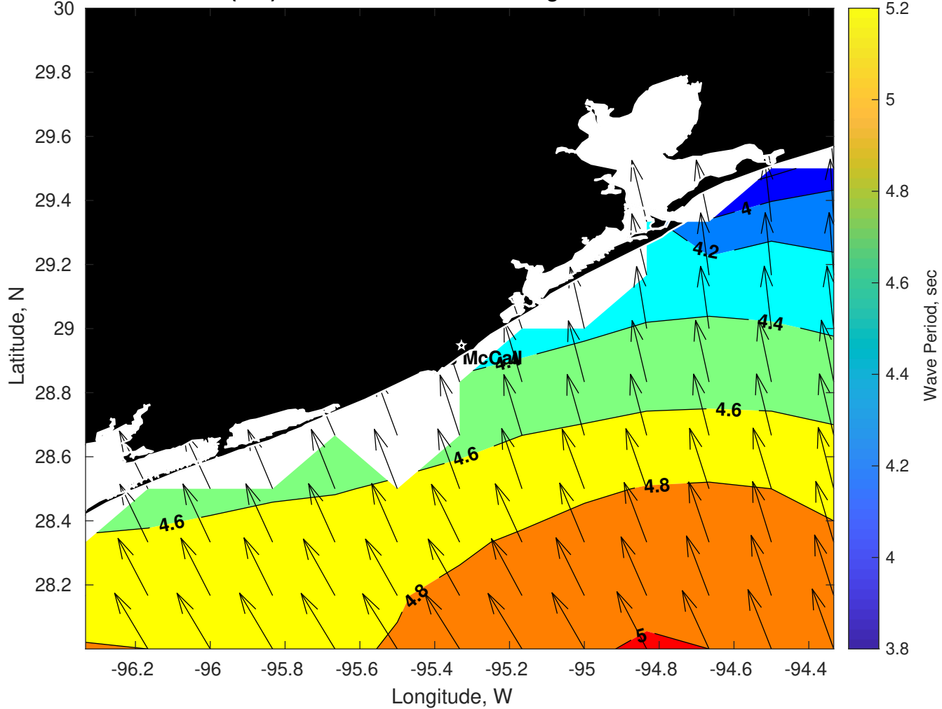
Wave Period (sec) for Brooks McCall at 15-Aug-2025 09:00:00
