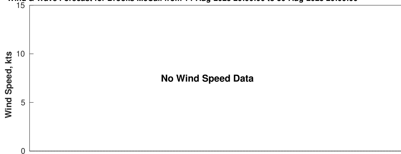
Wind & Wave Forecast for Brooks McCall from 14-Aug-2025 20:00:00 to 30-Aug-2025 20:00:00
