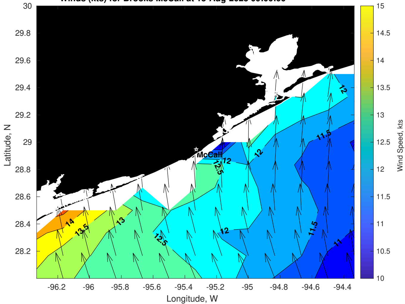
Winds (kts) for Brooks McCall at 15-Aug-2025 09:00:00
