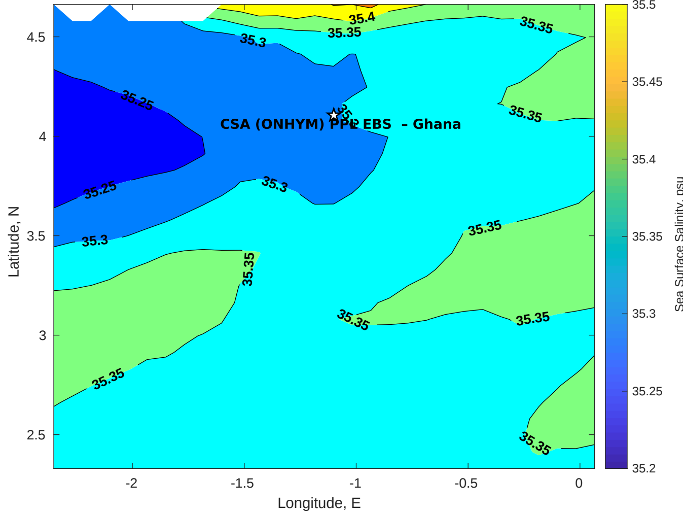
Surface Salinity for CSA (ONHYM) PPL EBS - Ghana at 14-Aug-2025 00:00:00
