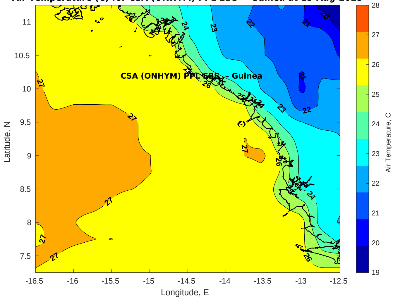
Air Temperature (C) for CSA (ONHYM) PPL EBS - Guinea at 15-Aug-2025
