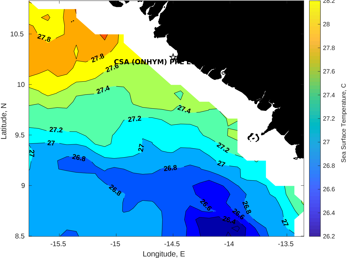
SST for CSA (ONHYM) PPL EBS - Guinea at 14-Aug-2025 00:00:00
