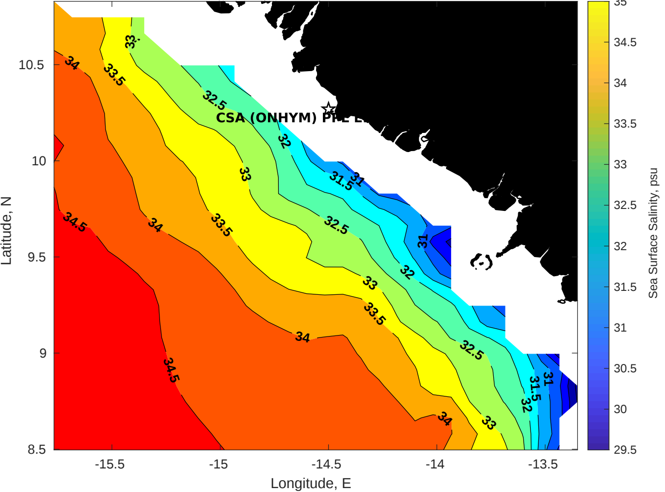
Surface Salinity for CSA (ONHYM) PPL EBS - Guinea at 14-Aug-2025 00:00:00
