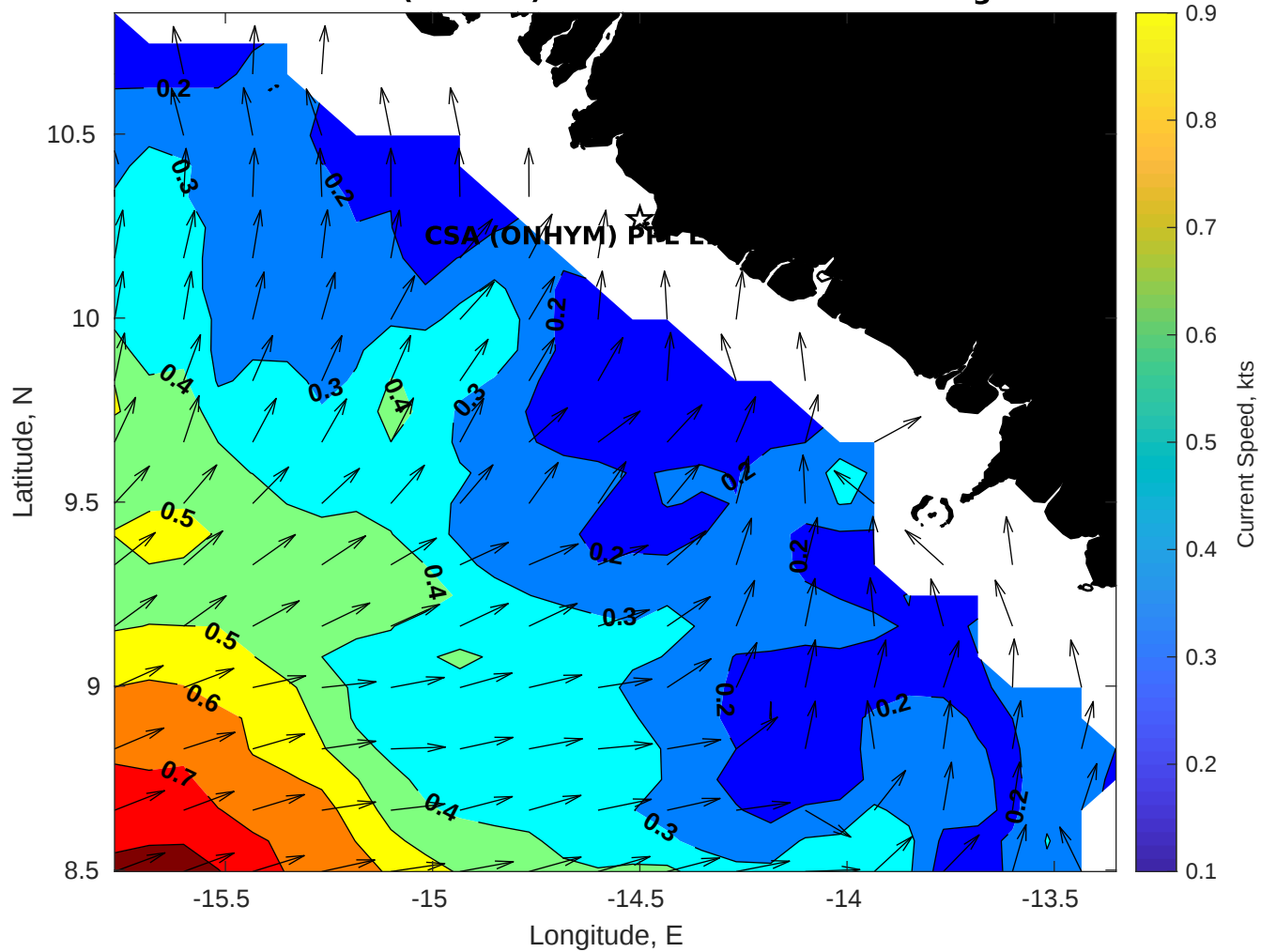
Surface Currents for CSA (ONHYM) PPL EBS - Guinea at 14-Aug-2025 00:00:00
