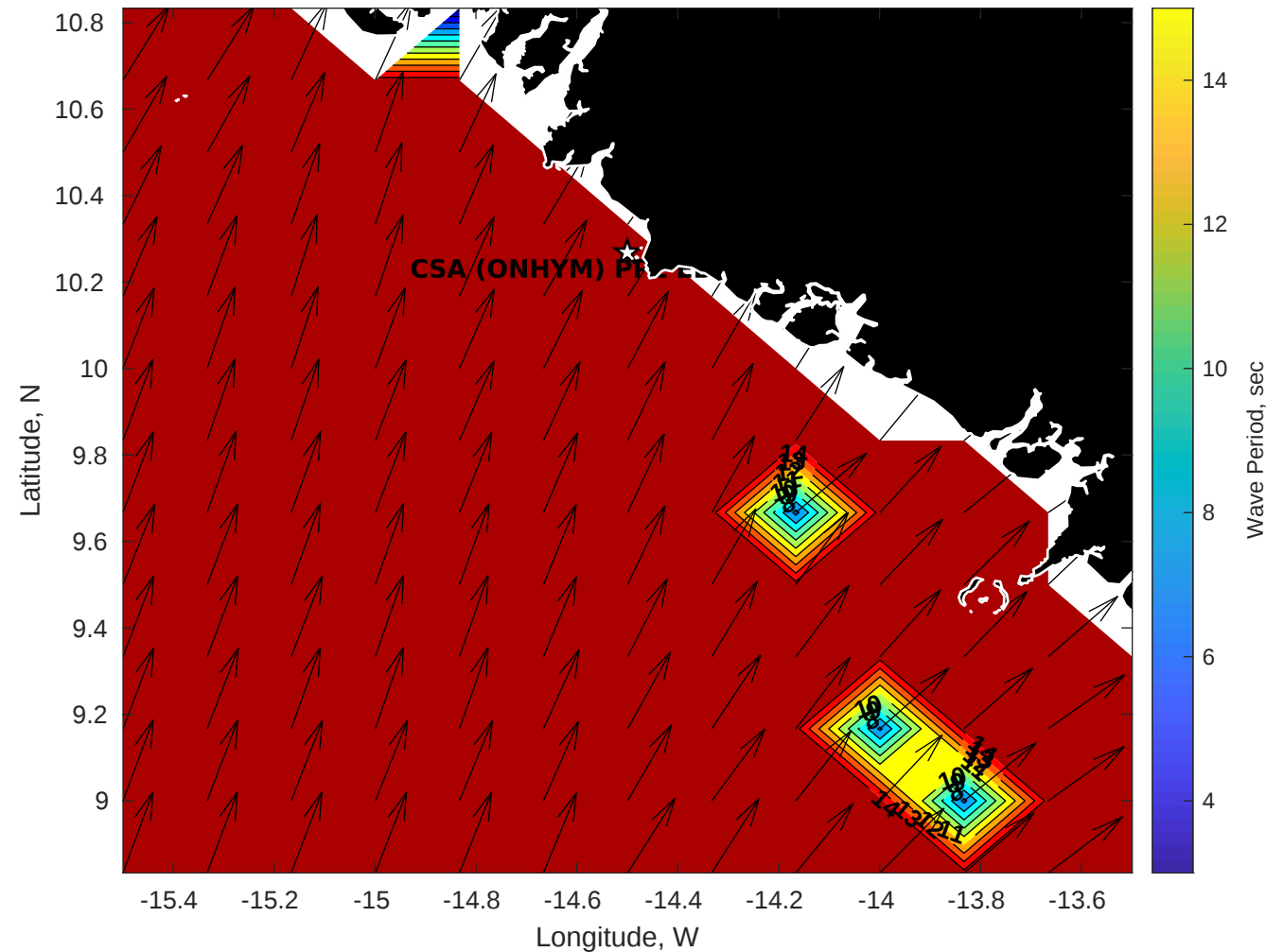
Wave Period (sec) for CSA (ONHYM) PPL EBS - Guinea at 15-Aug-2025 09:00:00
