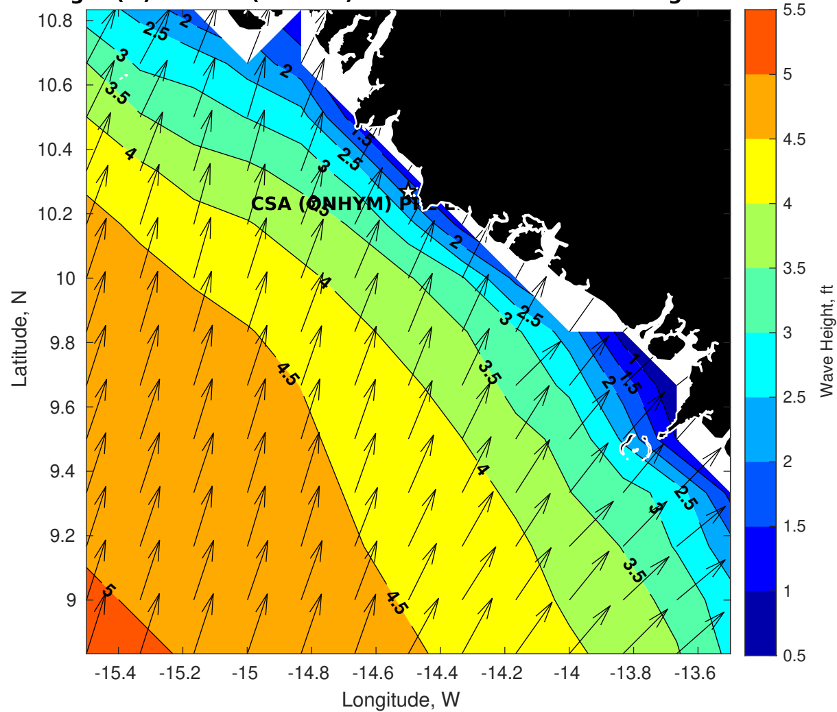
Wave Height (ft) for CSA (ONHYM) PPL EBS - Guinea at 15-Aug-2025 09:00:00
