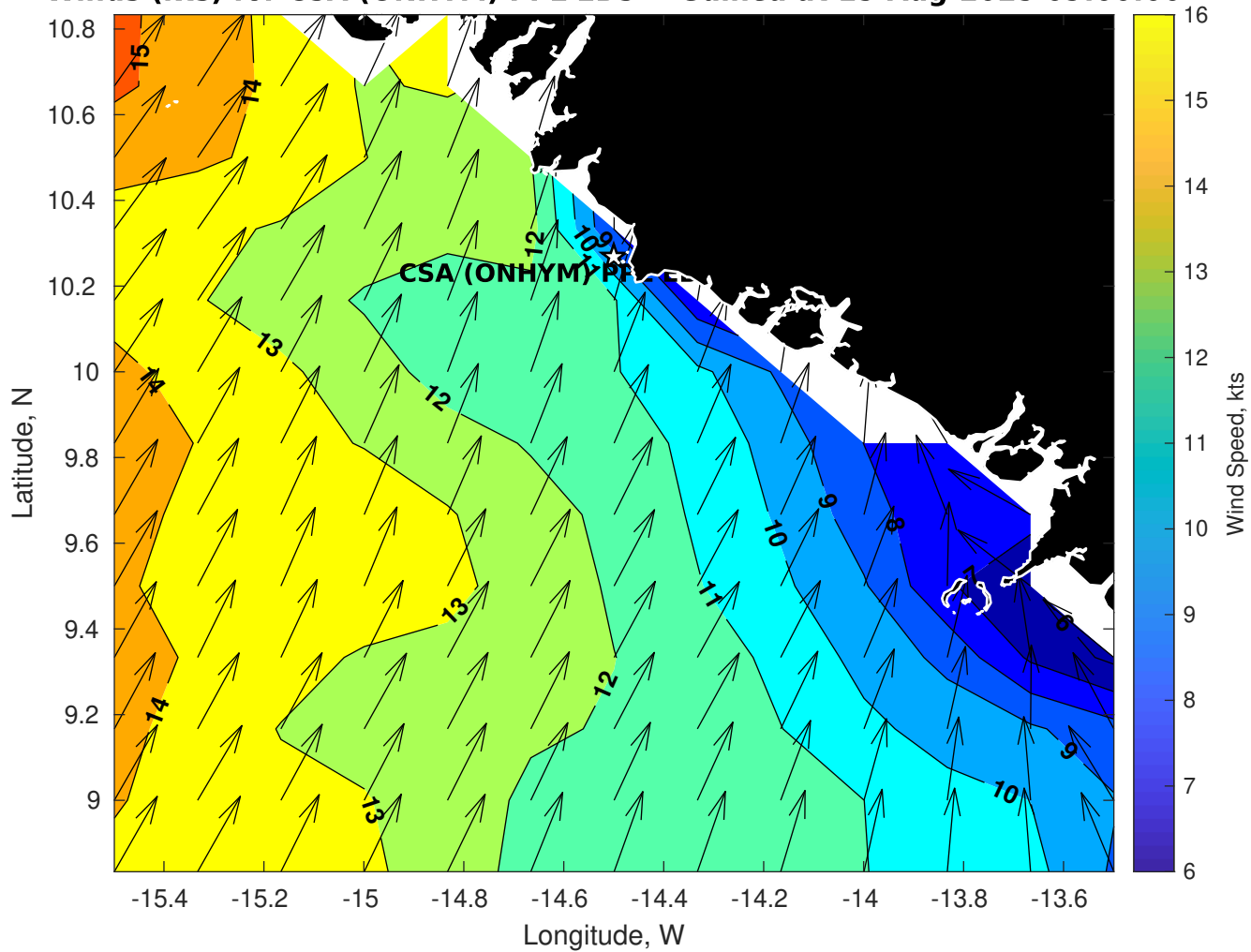
Winds (kts) for CSA (ONHYM) PPL EBS - Guinea at 15-Aug-2025 09:00:00
