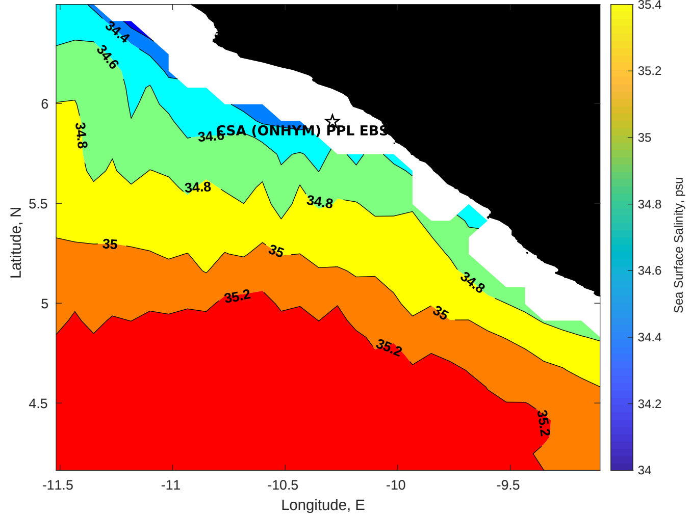
Surface Salinity for CSA (ONHYM) PPL EBS - Liberia at 14-Aug-2025 00:00:00
