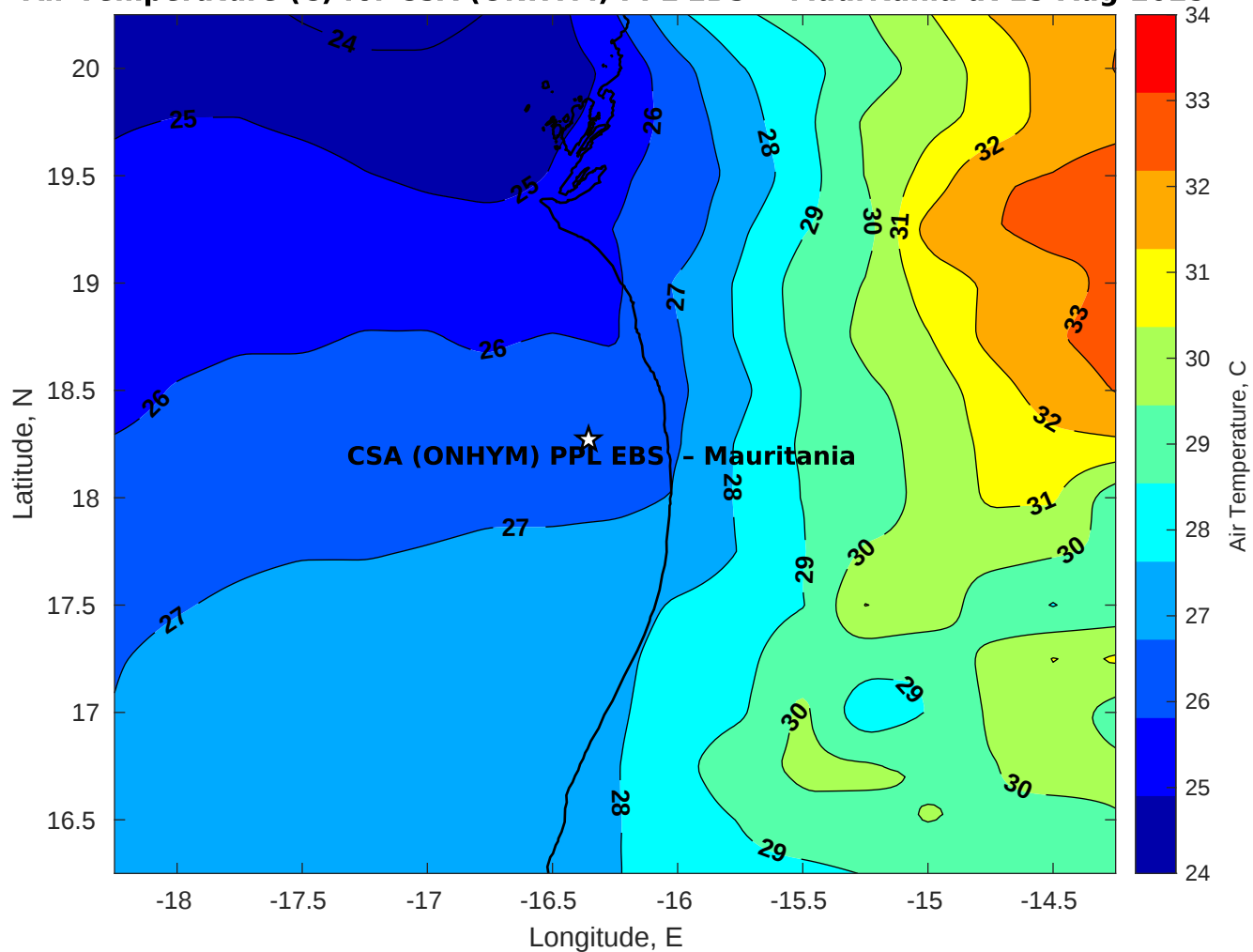
Air Temperature (C) for CSA (ONHYM) PPL EBS - Mauritania at 15-Aug-2025
