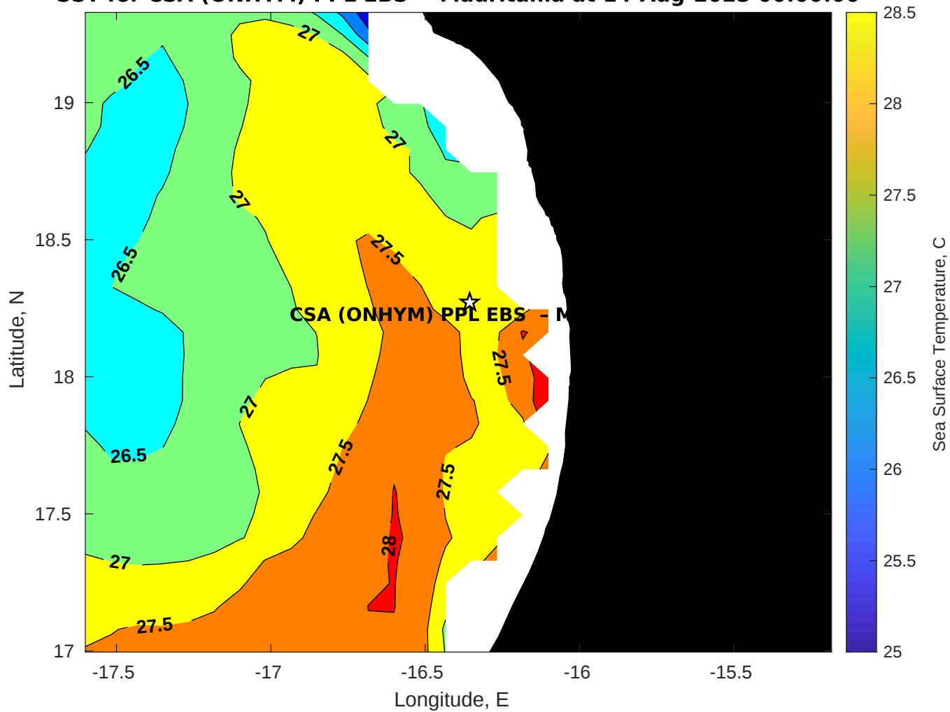
SST for CSA (ONHYM) PPL EBS - Mauritania at 14-Aug-2025 00:00:00
