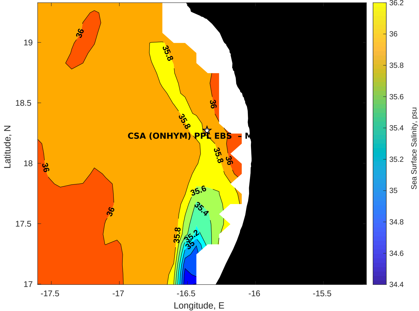
Surface Salinity for CSA (ONHYM) PPL EBS - Mauritania at 14-Aug-2025 00:00:00
