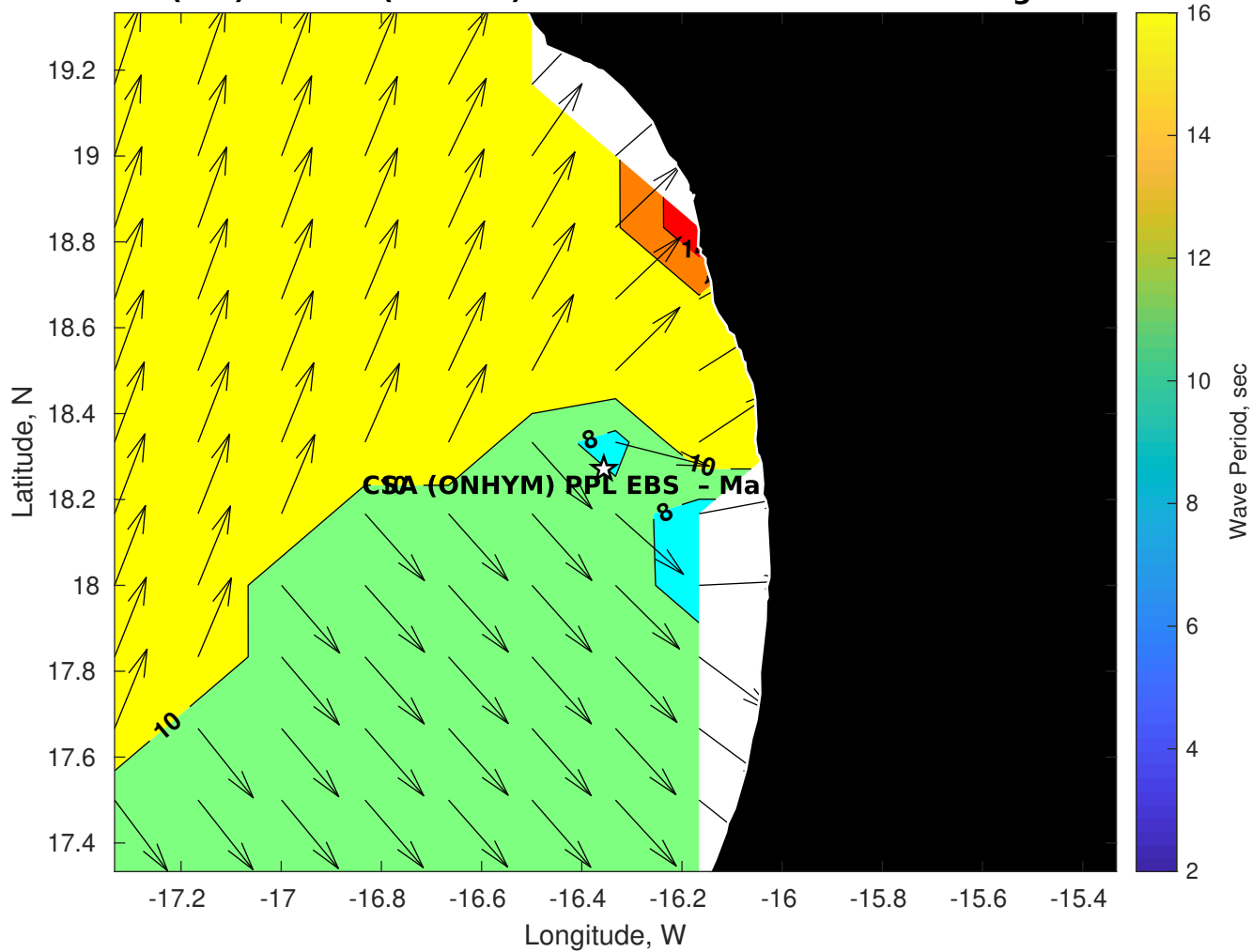
Wave Period (sec) for CSA (ONHYM) PPL EBS - Mauritania at 15-Aug-2025 09:00:00
