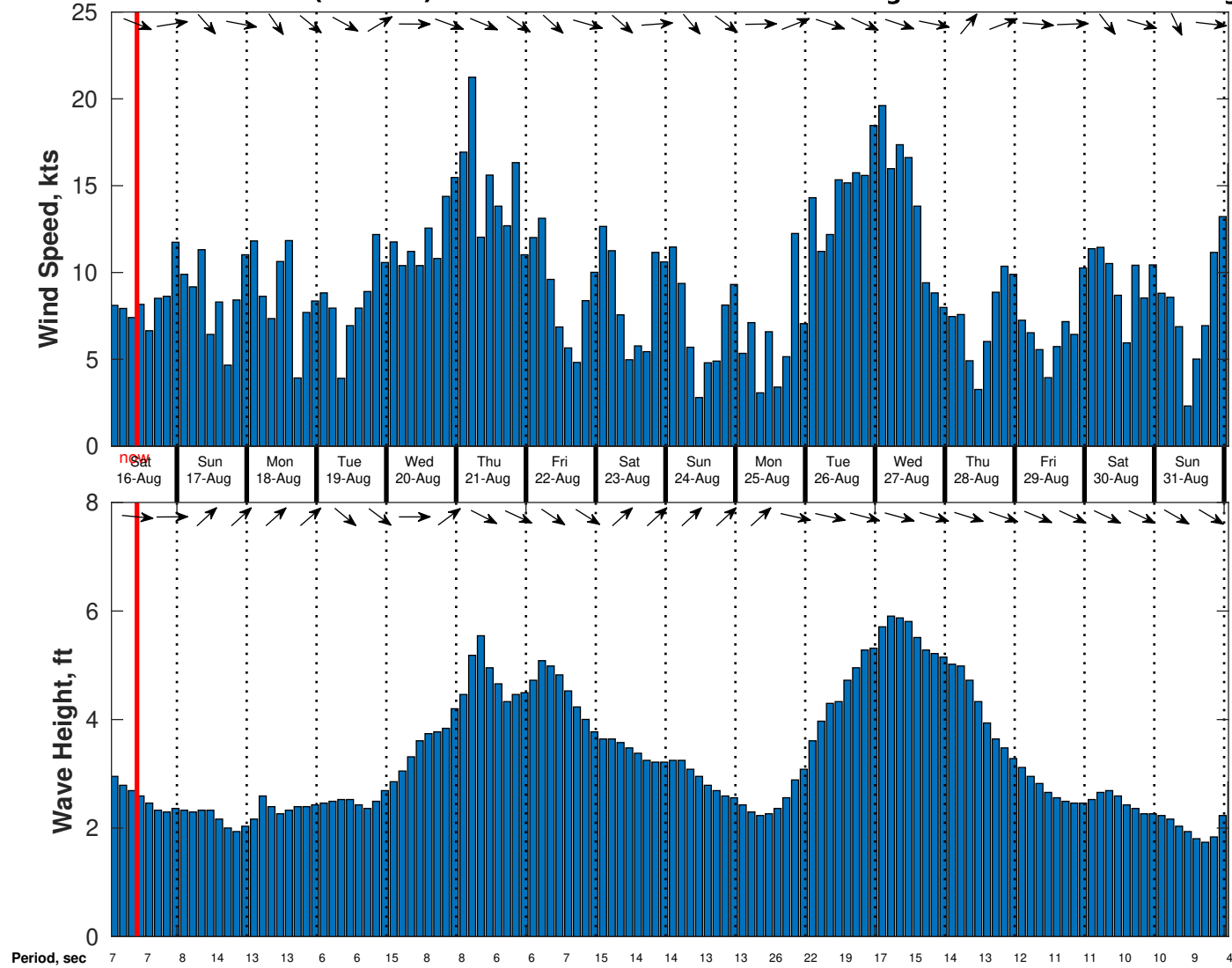
Wind & Wave Forecast for CSA (ONHYM) PPL EBS - Mauritania from 15-Aug-2025 01:00:00 to 31-Aug-2025 01:00:00
