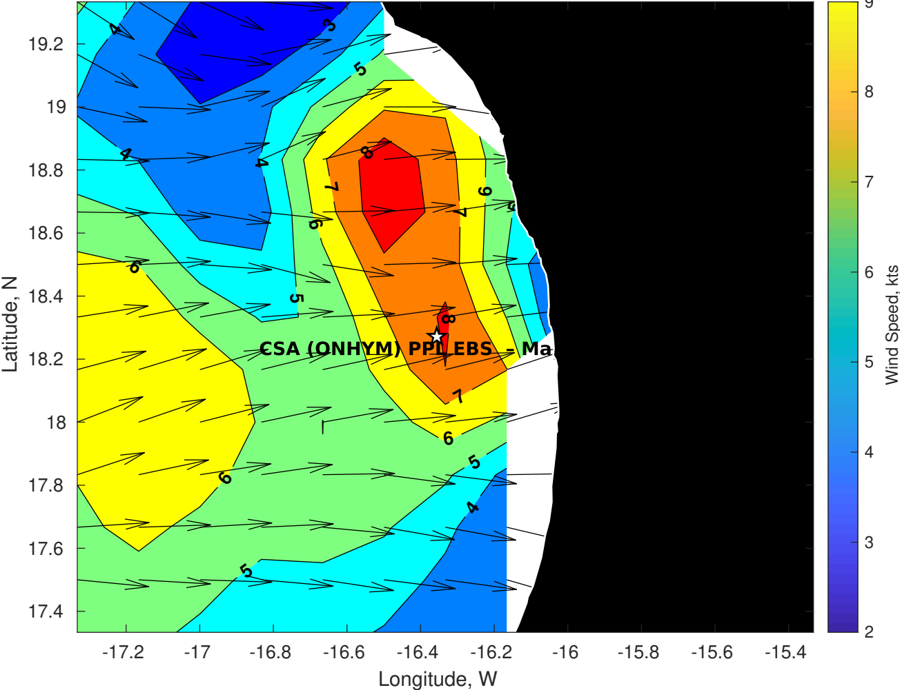
Winds (kts) for CSA (ONHYM) PPL EBS - Mauritania at 15-Aug-2025 09:00:00
