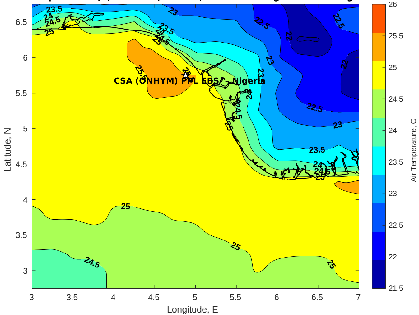
Air Temperature (C) for CSA (ONHYM) PPL EBS - Nigeria at 15-Aug-2025
