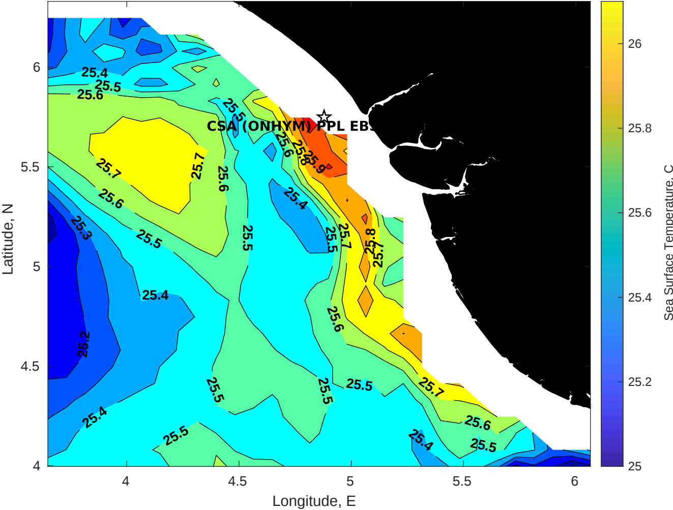
SST for CSA (ONHYM) PPL EBS - Nigeria at 14-Aug-2025 00:00:00
