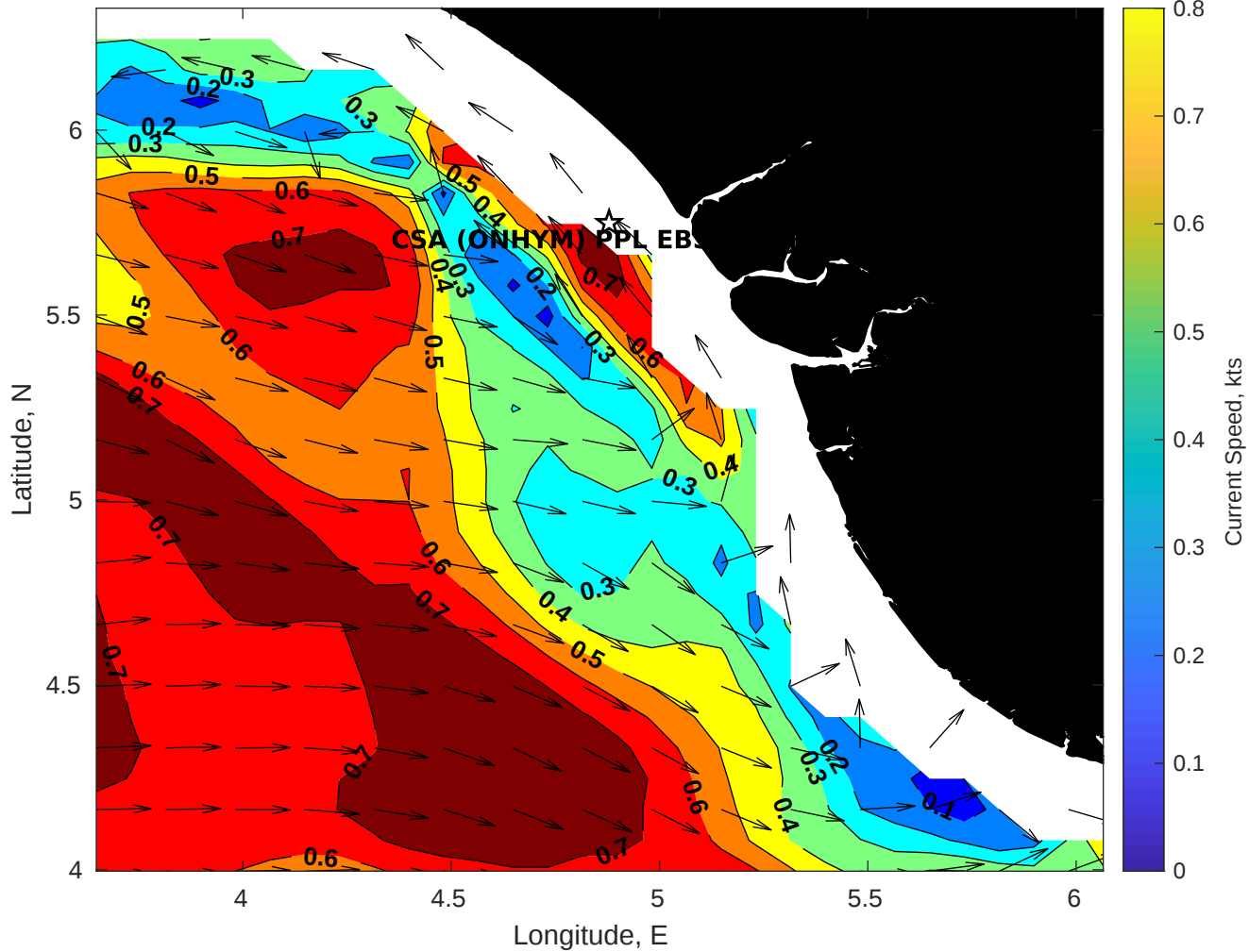
Surface Currents for CSA (ONHYM) PPL EBS - Nigeria at 14-Aug-2025 00:00:00
